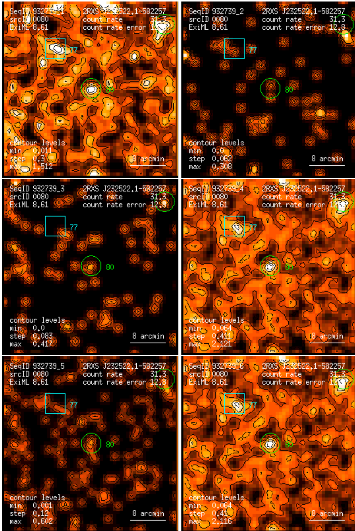
Figure 80: RASS 932739: detection 0080: band rate images, Gaussian filter: (1) PSPC channels 11 – 41, (2) 52 – 90, (3) 91 – 201, (4) 11 – 235, (5) 52 – 201, (6) 11 – 201. Broad band rates in counts/ks. Band rate contour levels in counts/ks/arcmin 2 .
