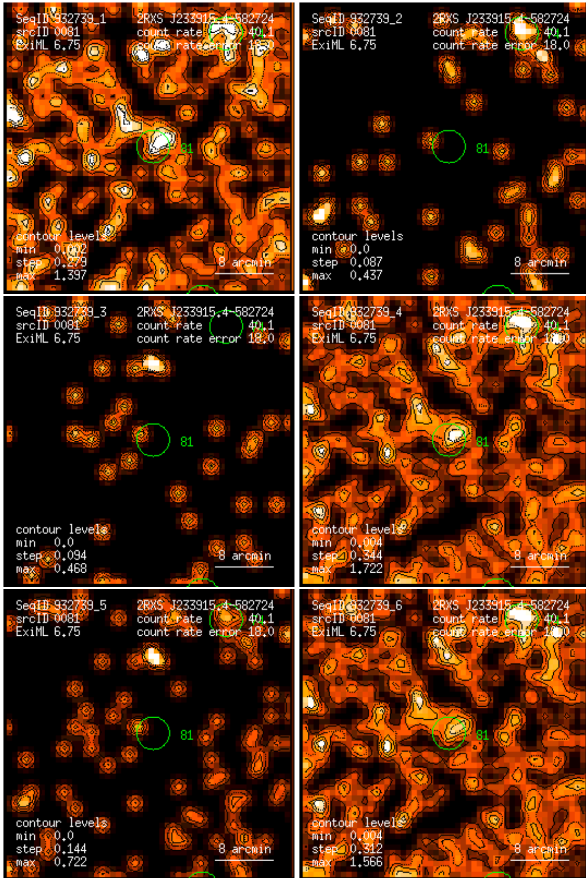
Figure 81: RASS 932739: detection 0081: band rate images, Gaussian filter: (1) PSPC channels 11 – 41, (2) 52 – 90, (3) 91 – 201, (4) 11 – 235, (5) 52 – 201, (6) 11 – 201. Broad band rates in counts/ks. Band rate contour levels in counts/ks/arcmin 2 .
