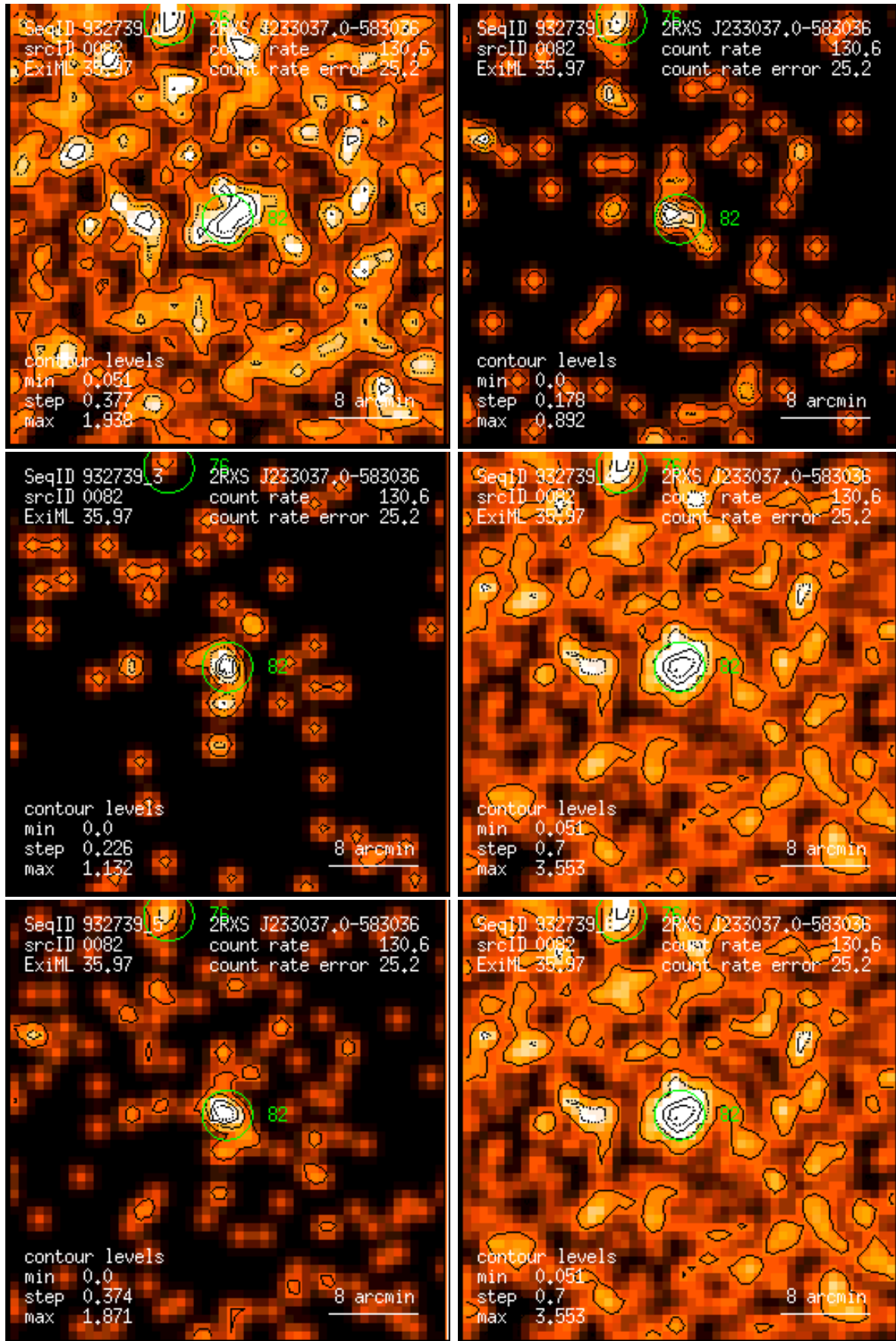
Figure 82: RASS 932739: detection 0082: band rate images, Gaussian filter: (1) PSPC channels 11 – 41, (2) 52 – 90, (3) 91 – 201, (4) 11 – 235, (5) 52 – 201, (6) 11 – 201. Broad band rates in counts/ks. Band rate contour levels in counts/ks/arcmin 2 .
