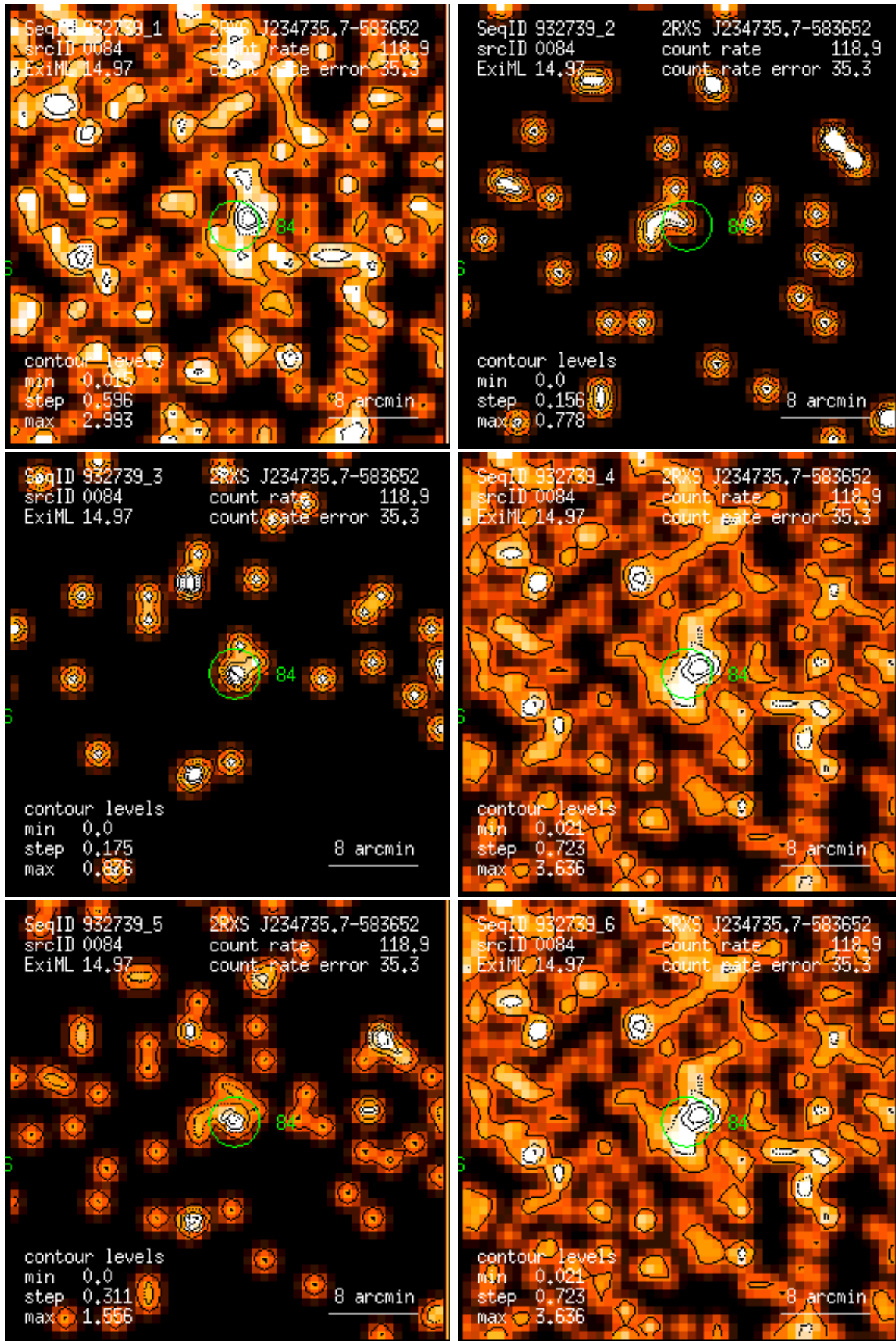
Figure 84: RASS 932739: detection 0084: band rate images, Gaussian filter: (1) PSPC channels 11 – 41, (2) 52 – 90, (3) 91 – 201, (4) 11 – 235, (5) 52 – 201, (6) 11 – 201. Broad band rates in counts/ks. Band rate contour levels in counts/ks/arcmin 2 .
