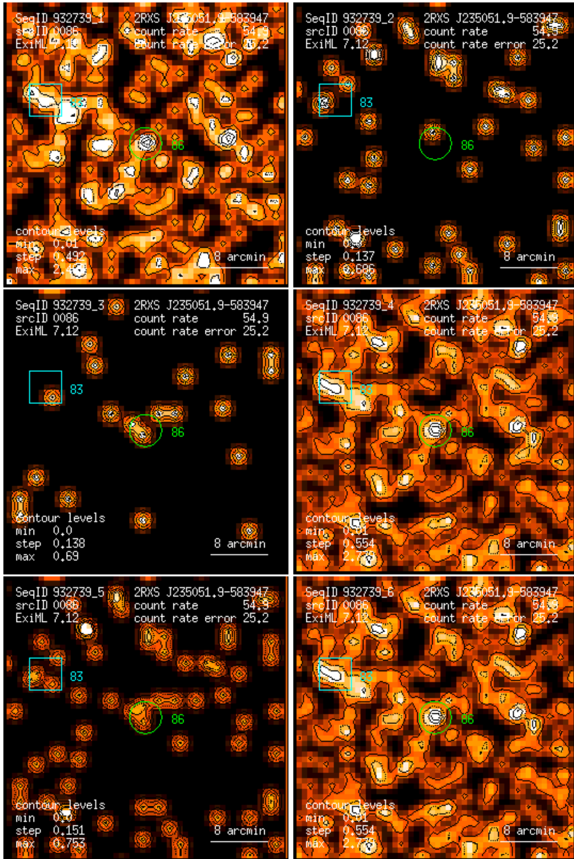
Figure 86: RASS 932739: detection 0086: band rate images, Gaussian filter: (1) PSPC channels 11 – 41, (2) 52 – 90, (3) 91 – 201, (4) 11 – 235, (5) 52 – 201, (6) 11 – 201. Broad band rates in counts/ks. Band rate contour levels in counts/ks/arcmin 2 .
