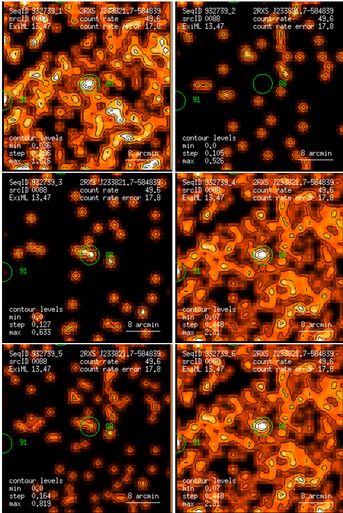
Figure 88: RASS 932739: detection 0088: band rate images, Gaussian filter: (1) PSPC channels 11 – 41, (2) 52 – 90, (3) 91 – 201, (4) 11 – 235, (5) 52 – 201, (6) 11 – 201. Broad band rates in counts/ks. Band rate contour levels in counts/ks/arcmin 2 .
