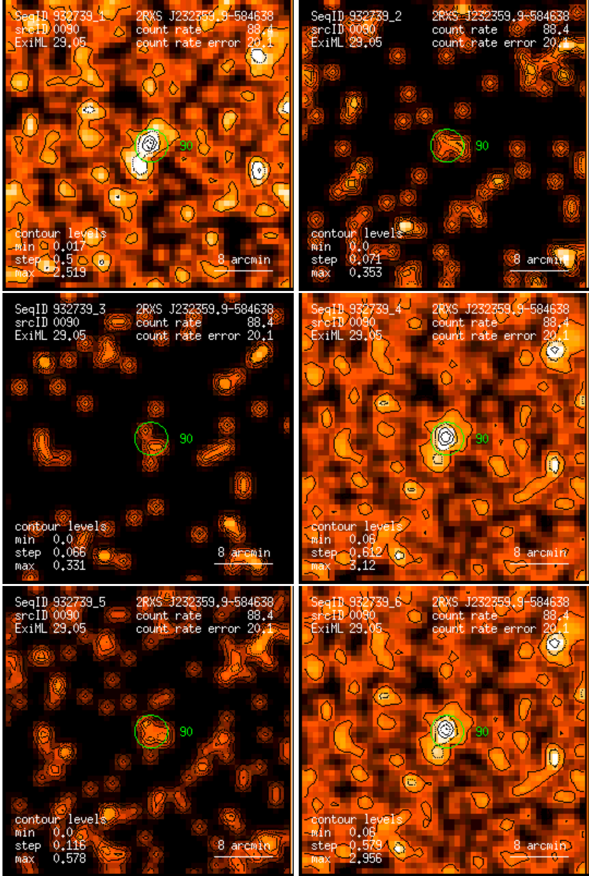
Figure 90: RASS 932739: detection 0090: band rate images, Gaussian filter: (1) PSPC channels 11 – 41, (2) 52 – 90, (3) 91 – 201, (4) 11 – 235, (5) 52 – 201, (6) 11 – 201. Broad band rates in counts/ks. Band rate contour levels in counts/ks/arcmin 2 .
