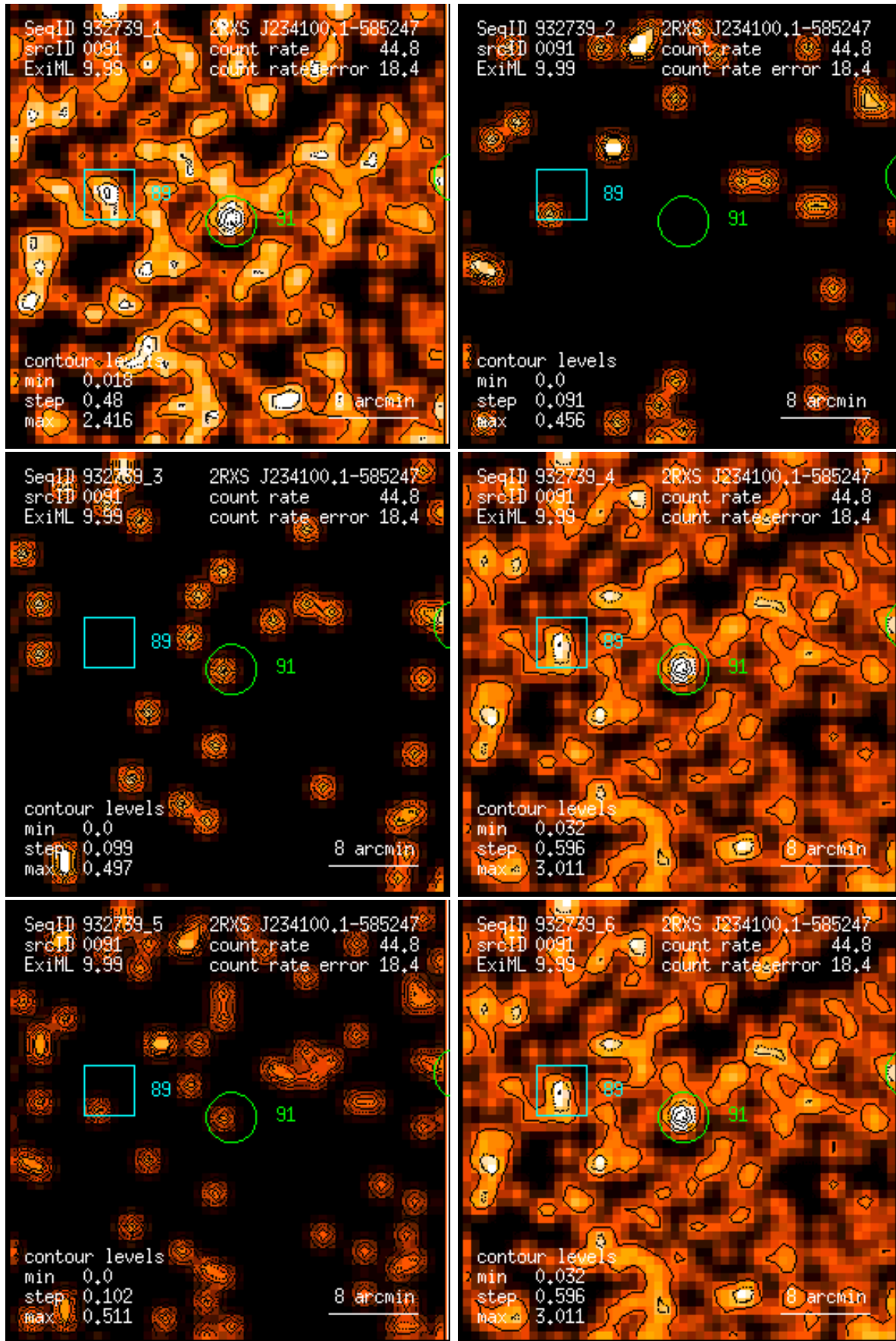
Figure 91: RASS 932739: detection 0091: band rate images, Gaussian filter: (1) PSPC channels 11 – 41, (2) 52 – 90, (3) 91 – 201, (4) 11 – 235, (5) 52 – 201, (6) 11 – 201. Broad band rates in counts/ks. Band rate contour levels in counts/ks/arcmin 2 .
