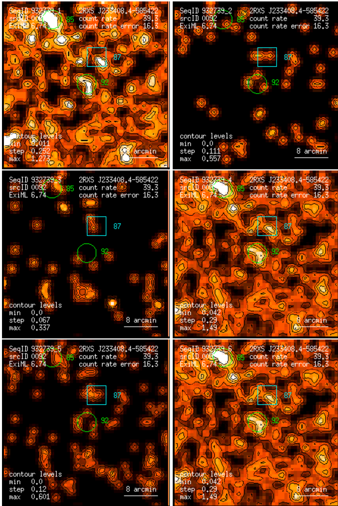
Figure 92: RASS 932739: detection 0092: band rate images, Gaussian filter: (1) PSPC channels 11 – 41, (2) 52 – 90, (3) 91 – 201, (4) 11 – 235, (5) 52 – 201, (6) 11 – 201. Broad band rates in counts/ks. Band rate contour levels in counts/ks/arcmin 2 .
