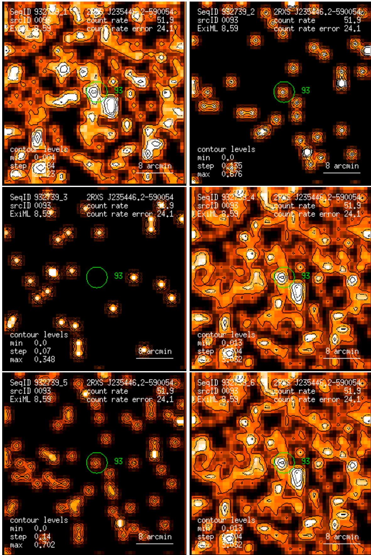
Figure 93: RASS 932739: detection 0093: band rate images, Gaussian filter: (1) PSPC channels 11 – 41, (2) 52 – 90, (3) 91 – 201, (4) 11 – 235, (5) 52 – 201, (6) 11 – 201. Broad band rates in counts/ks. Band rate contour levels in counts/ks/arcmin 2 .
