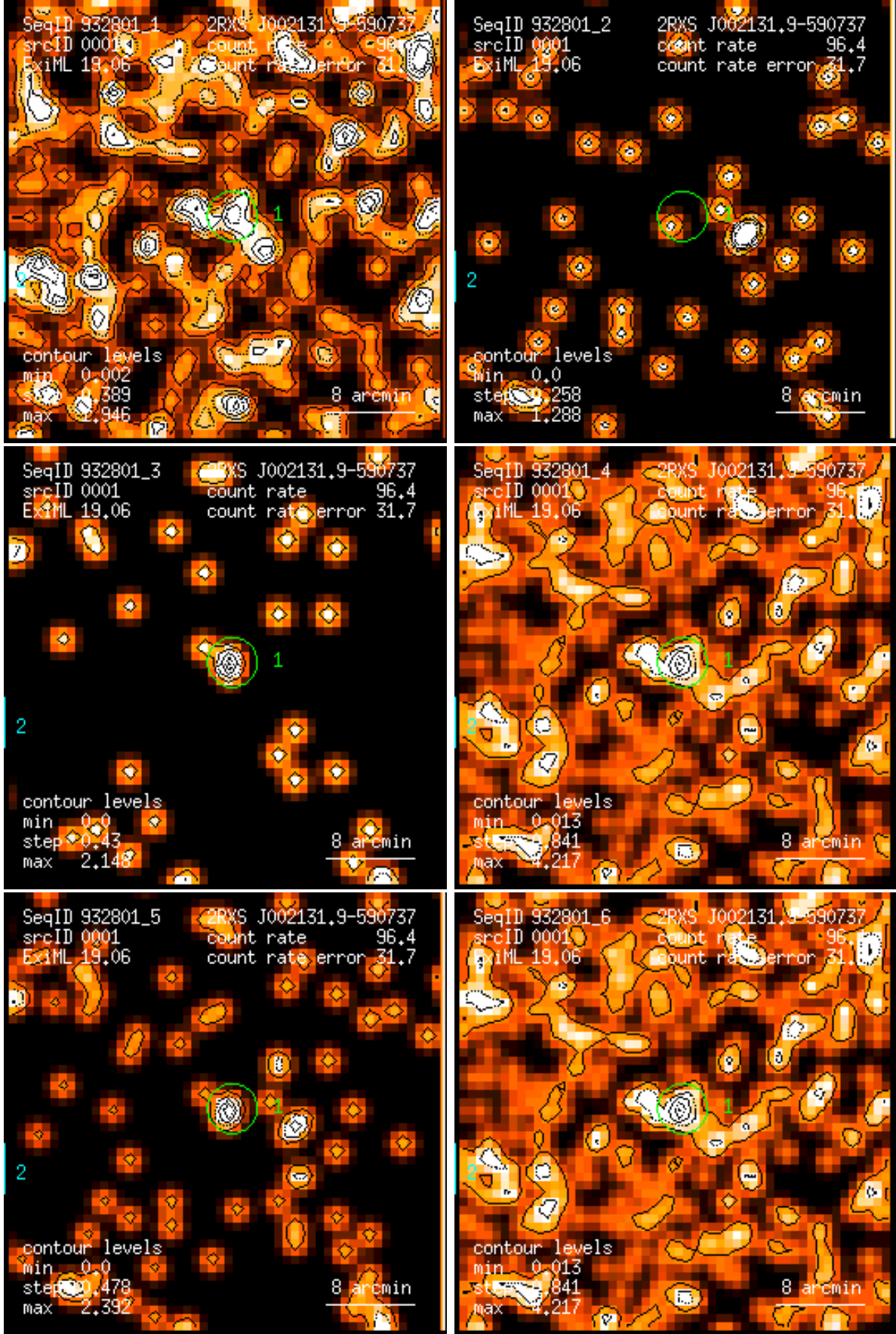
Figure 1: RASS 932801: detection 0001: band rate images, Gaussian filter: (1) PSPC channels 11 – 41, (2) 52 – 90, (3) 91 – 201, (4) 11 – 235, (5) 52 – 201, (6) 11 – 201. Broad band rates in counts/ks. Band rate contour levels in counts/ks/arcmin 2 .
