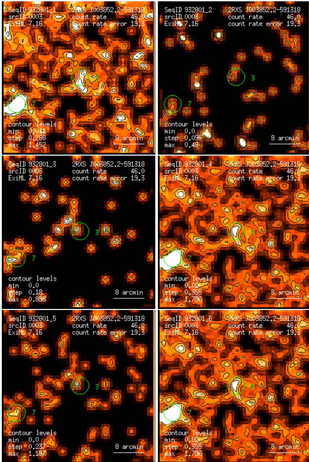
Figure 3: RASS 932801: detection 0003: band rate images, Gaussian filter: (1) PSPC channels 11 – 41, (2) 52 – 90, (3) 91 – 201, (4) 11 – 235, (5) 52 – 201, (6) 11 – 201. Broad band rates in counts/ks. Band rate contour levels in counts/ks/arcmin 2 .
