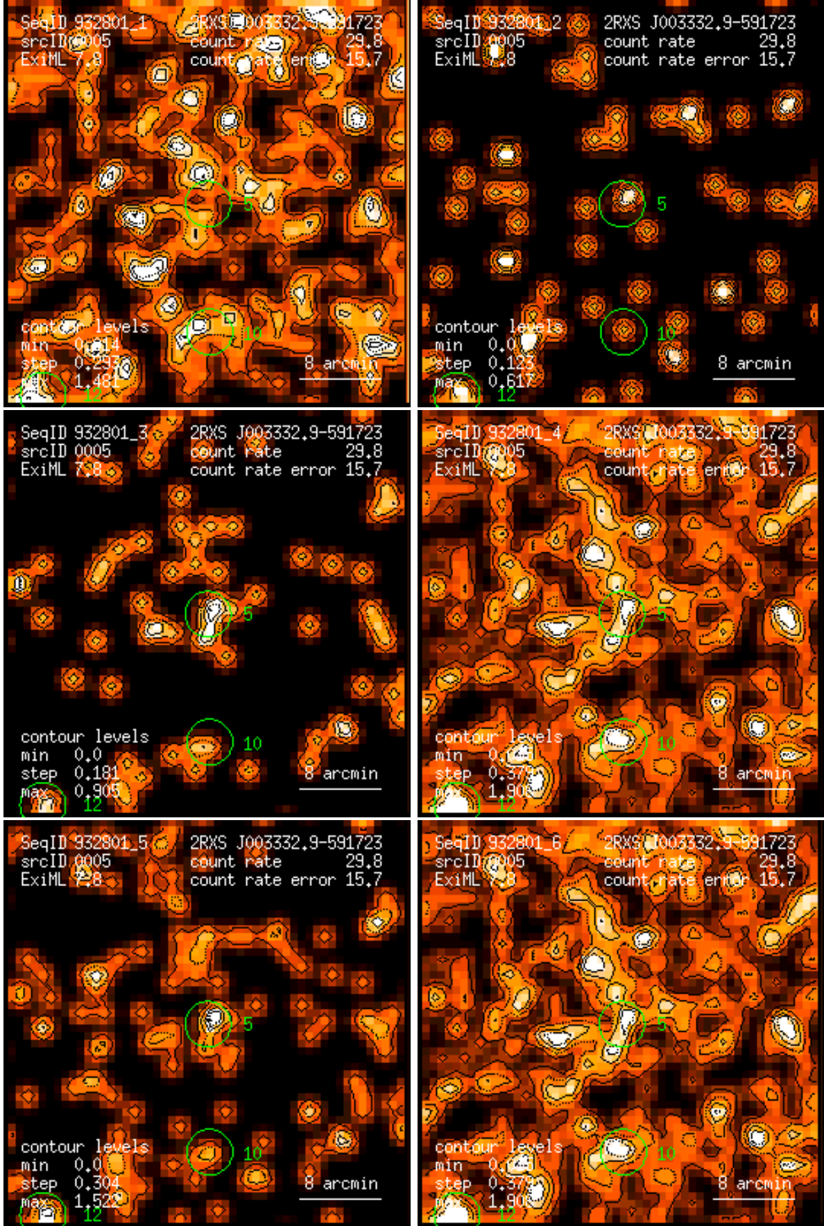
Figure 5: RASS 932801: detection 0005: band rate images, Gaussian filter: (1) PSPC channels 11 – 41, (2) 52 – 90, (3) 91 – 201, (4) 11 – 235, (5) 52 – 201, (6) 11 – 201. Broad band rates in counts/ks. Band rate contour levels in counts/ks/arcmin 2 .
