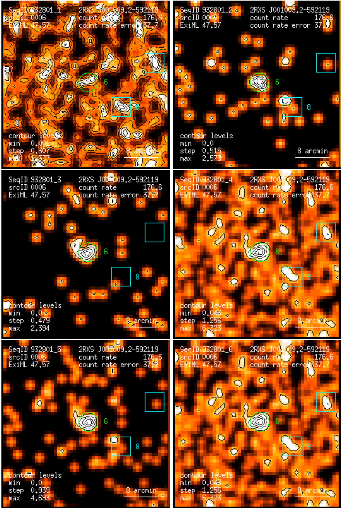
Figure 6: RASS 932801: detection 0006: band rate images, Gaussian filter: (1) PSPC channels 11 – 41, (2) 52 – 90, (3) 91 – 201, (4) 11 – 235, (5) 52 – 201, (6) 11 – 201. Broad band rates in counts/ks. Band rate contour levels in counts/ks/arcmin 2 .
