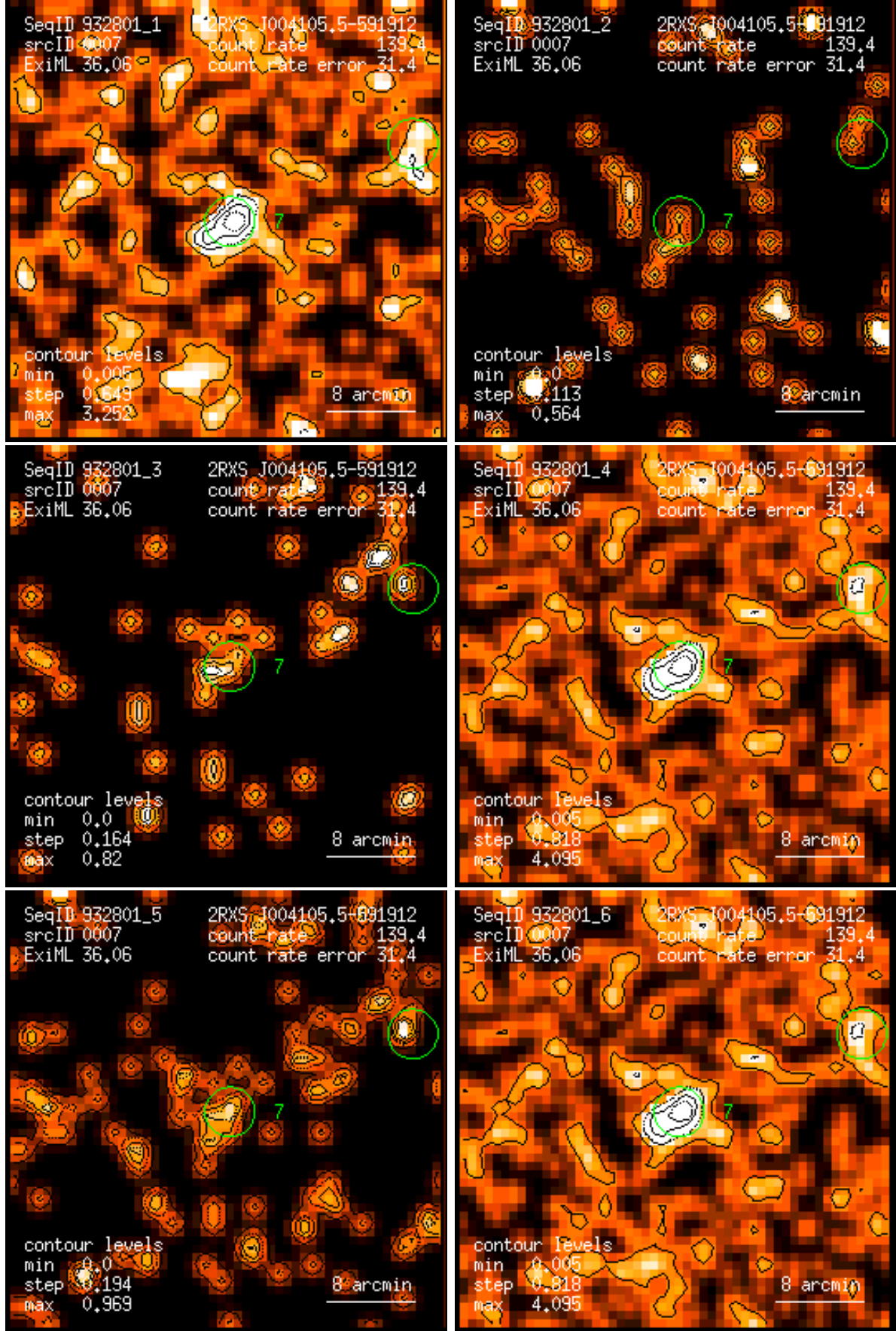
Figure 7: RASS 932801: detection 0007: band rate images, Gaussian filter: (1) PSPC channels 11 – 41, (2) 52 – 90, (3) 91 – 201, (4) 11 – 235, (5) 52 – 201, (6) 11 – 201. Broad band rates in counts/ks. Band rate contour levels in counts/ks/arcmin 2 .
