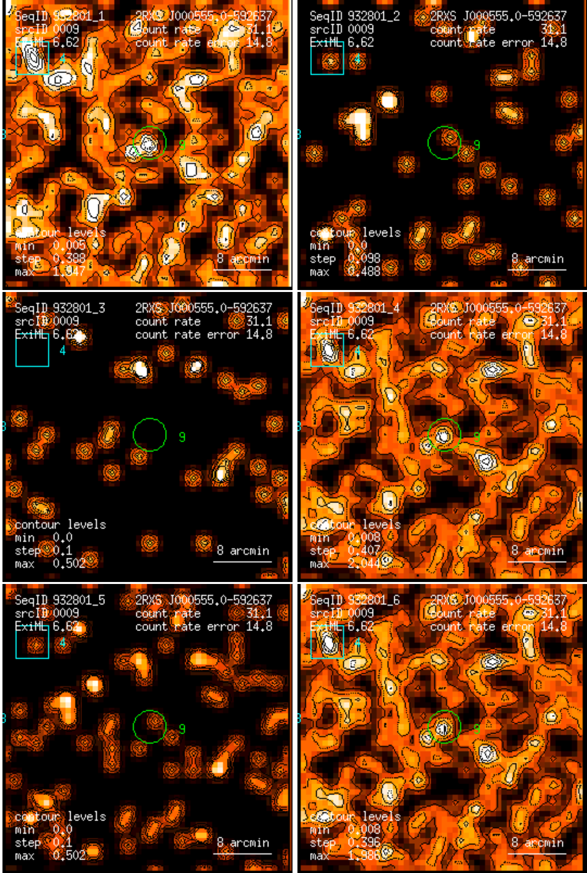
Figure 9: RASS 932801: detection 0009: band rate images, Gaussian filter: (1) PSPC channels 11 – 41, (2) 52 – 90, (3) 91 – 201, (4) 11 – 235, (5) 52 – 201, (6) 11 – 201. Broad band rates in counts/ks. Band rate contour levels in counts/ks/arcmin 2 .
