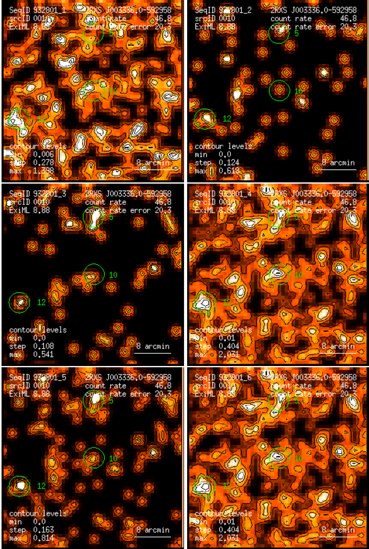
Figure 10: RASS 932801: detection 0010: band rate images, Gaussian filter: (1) PSPC channels 11 – 41, (2) 52 – 90, (3) 91 – 201, (4) 11 – 235, (5) 52 – 201, (6) 11 – 201. Broad band rates in counts/ks. Band rate contour levels in counts/ks/arcmin 2 .
