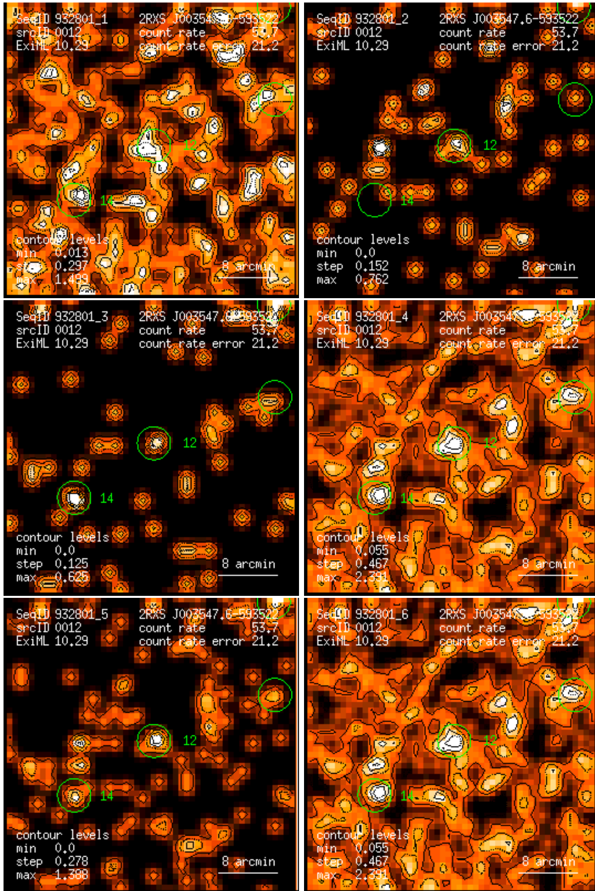
Figure 12: RASS 932801: detection 0012: band rate images, Gaussian filter: (1) PSPC channels 11 – 41, (2) 52 – 90, (3) 91 – 201, (4) 11 – 235, (5) 52 – 201, (6) 11 – 201. Broad band rates in counts/ks. Band rate contour levels in counts/ks/arcmin 2 .
