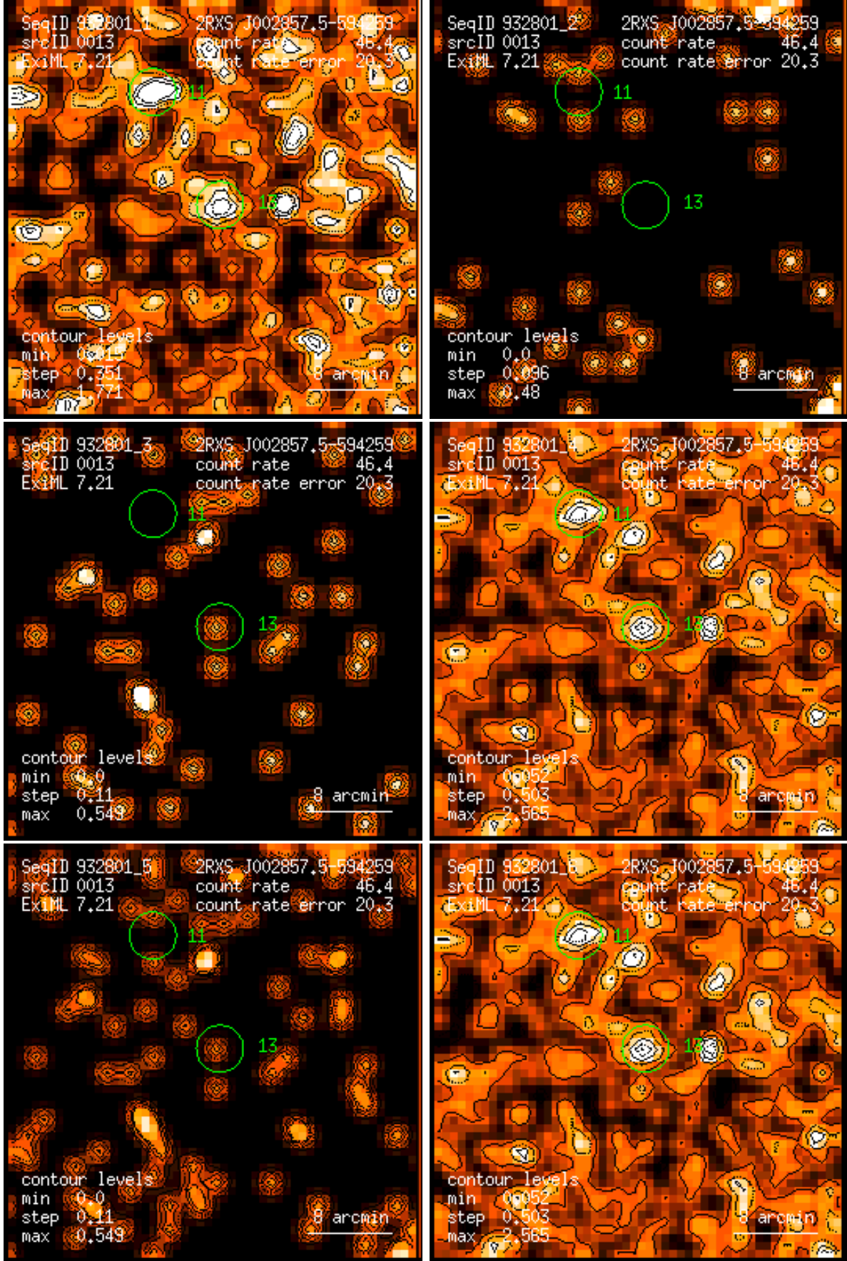
Figure 13: RASS 932801: detection 0013: band rate images, Gaussian filter: (1) PSPC channels 11 – 41, (2) 52 – 90, (3) 91 – 201, (4) 11 – 235, (5) 52 – 201, (6) 11 – 201. Broad band rates in counts/ks. Band rate contour levels in counts/ks/arcmin 2 .
