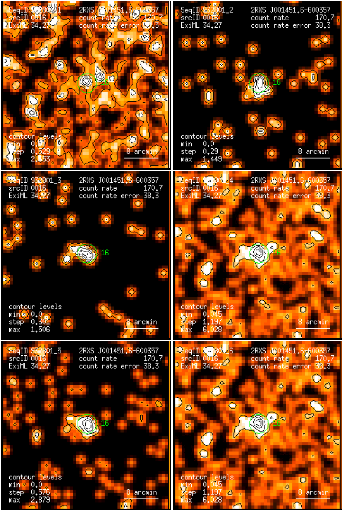
Figure 16: RASS 932801: detection 0016: band rate images, Gaussian filter: (1) PSPC channels 11 – 41, (2) 52 – 90, (3) 91 – 201, (4) 11 – 235, (5) 52 – 201, (6) 11 – 201. Broad band rates in counts/ks. Band rate contour levels in counts/ks/arcmin 2 .
