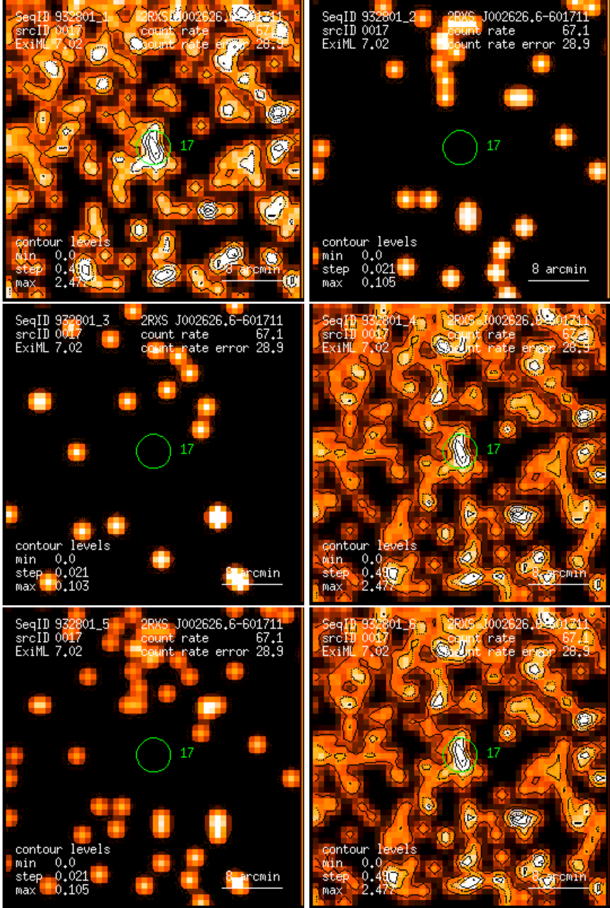
Figure 17: RASS 932801: detection 0017: band rate images, Gaussian filter: (1) PSPC channels 11 – 41, (2) 52 – 90, (3) 91 – 201, (4) 11 – 235, (5) 52 – 201, (6) 11 – 201. Broad band rates in counts/ks. Band rate contour levels in counts/ks/arcmin 2 .
