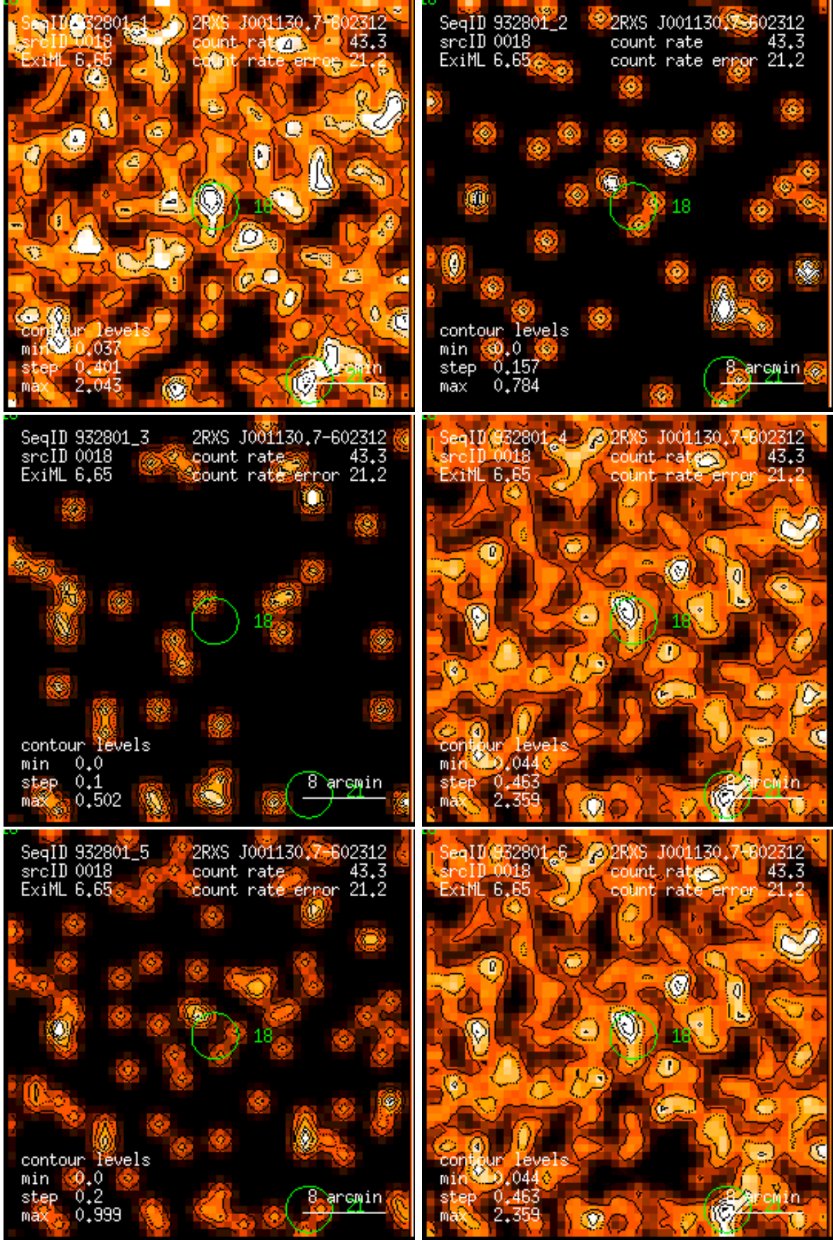
Figure 18: RASS 932801: detection 0018: band rate images, Gaussian filter: (1) PSPC channels 11 – 41, (2) 52 – 90, (3) 91 – 201, (4) 11 – 235, (5) 52 – 201, (6) 11 – 201. Broad band rates in counts/ks. Band rate contour levels in counts/ks/arcmin 2 .
