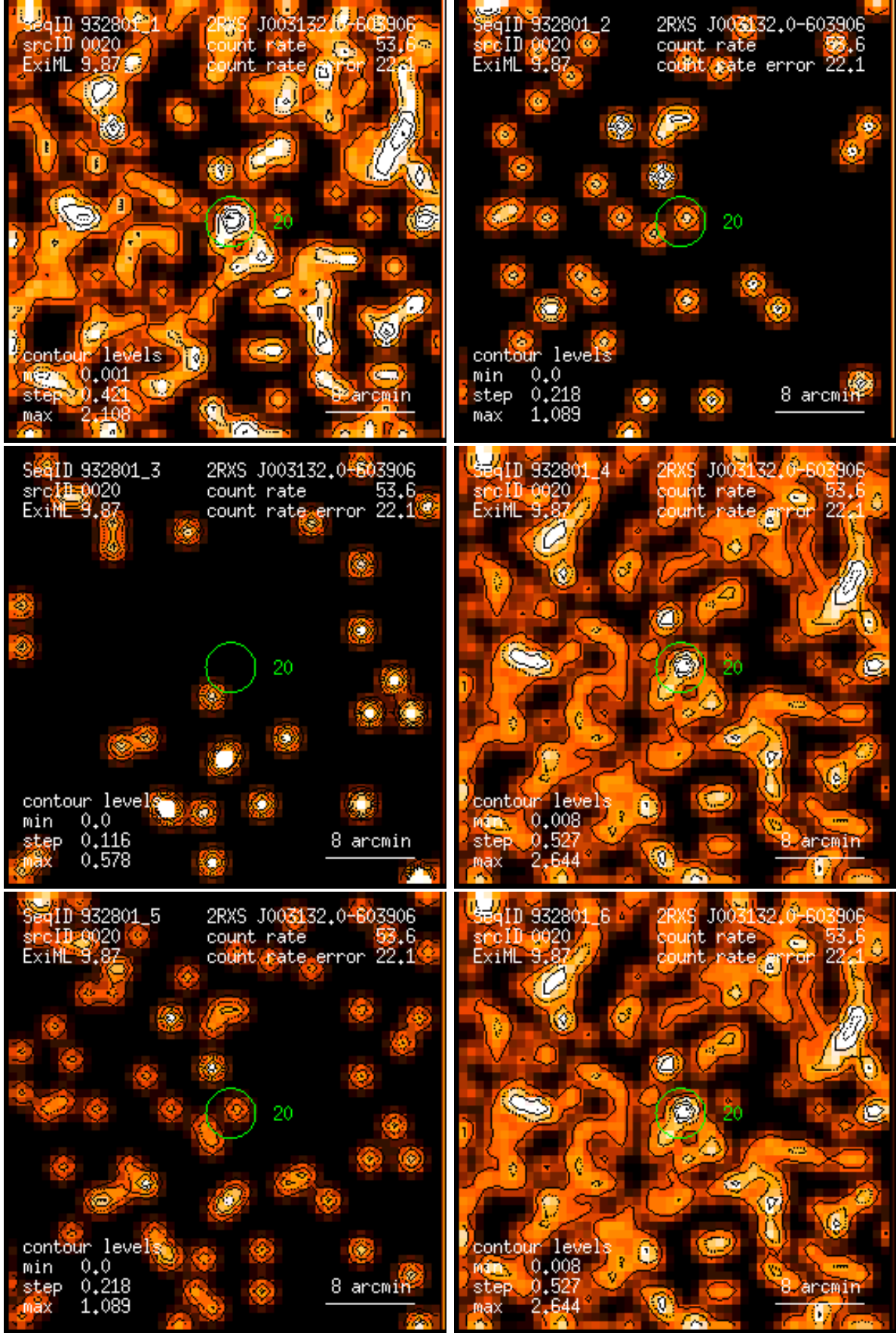
Figure 20: RASS 932801: detection 0020: band rate images, Gaussian filter: (1) PSPC channels 11 – 41, (2) 52 – 90, (3) 91 – 201, (4) 11 – 235, (5) 52 – 201, (6) 11 – 201. Broad band rates in counts/ks. Band rate contour levels in counts/ks/arcmin 2 .
