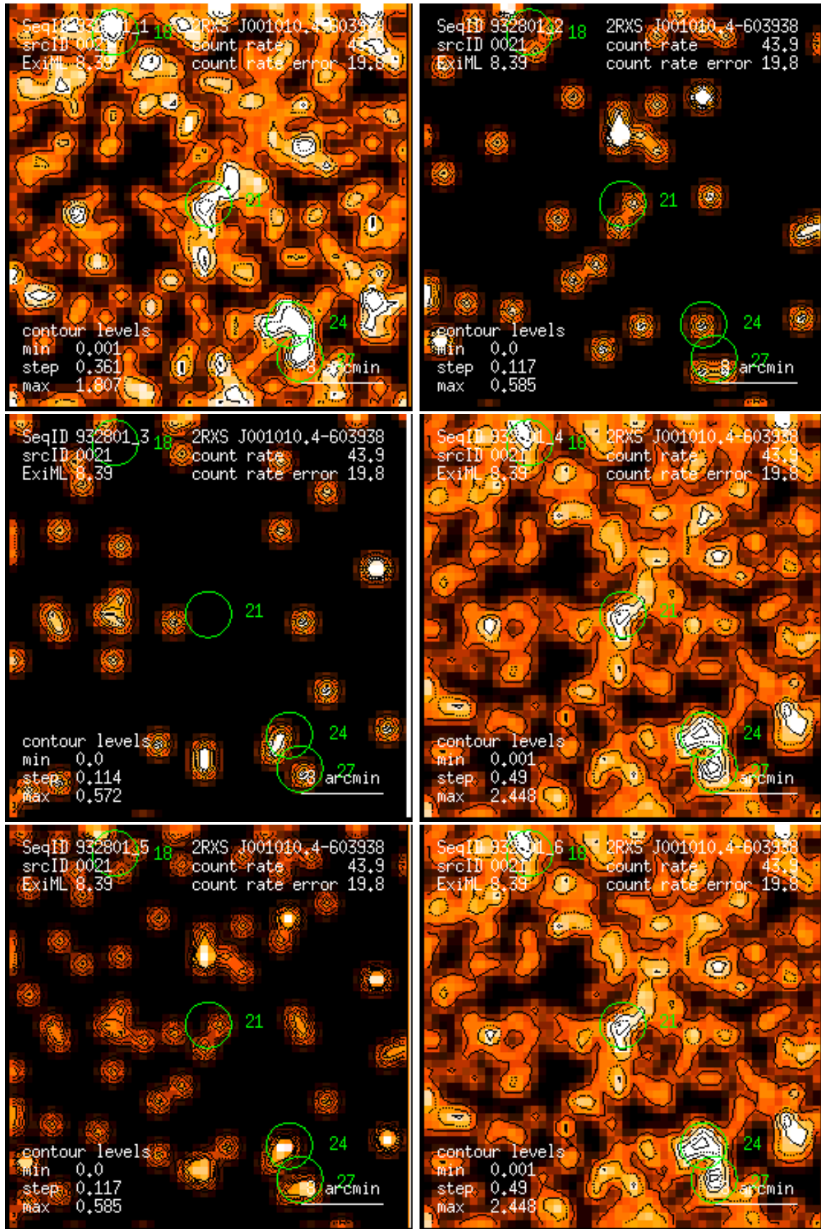
Figure 21: RASS 932801: detection 0021: band rate images, Gaussian filter: (1) PSPC channels 11 – 41, (2) 52 – 90, (3) 91 – 201, (4) 11 – 235, (5) 52 – 201, (6) 11 – 201. Broad band rates in counts/ks. Band rate contour levels in counts/ks/arcmin 2 .
