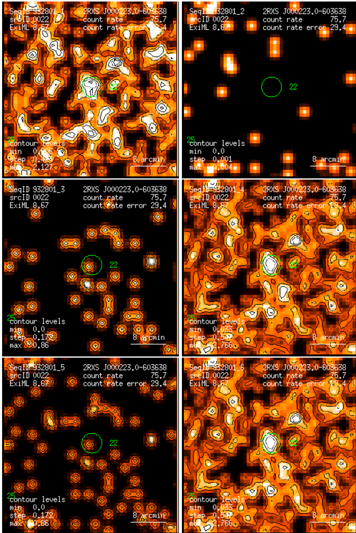
Figure 22: RASS 932801: detection 0022: band rate images, Gaussian filter: (1) PSPC channels 11 – 41, (2) 52 – 90, (3) 91 – 201, (4) 11 – 235, (5) 52 – 201, (6) 11 – 201. Broad band rates in counts/ks. Band rate contour levels in counts/ks/arcmin 2 .
