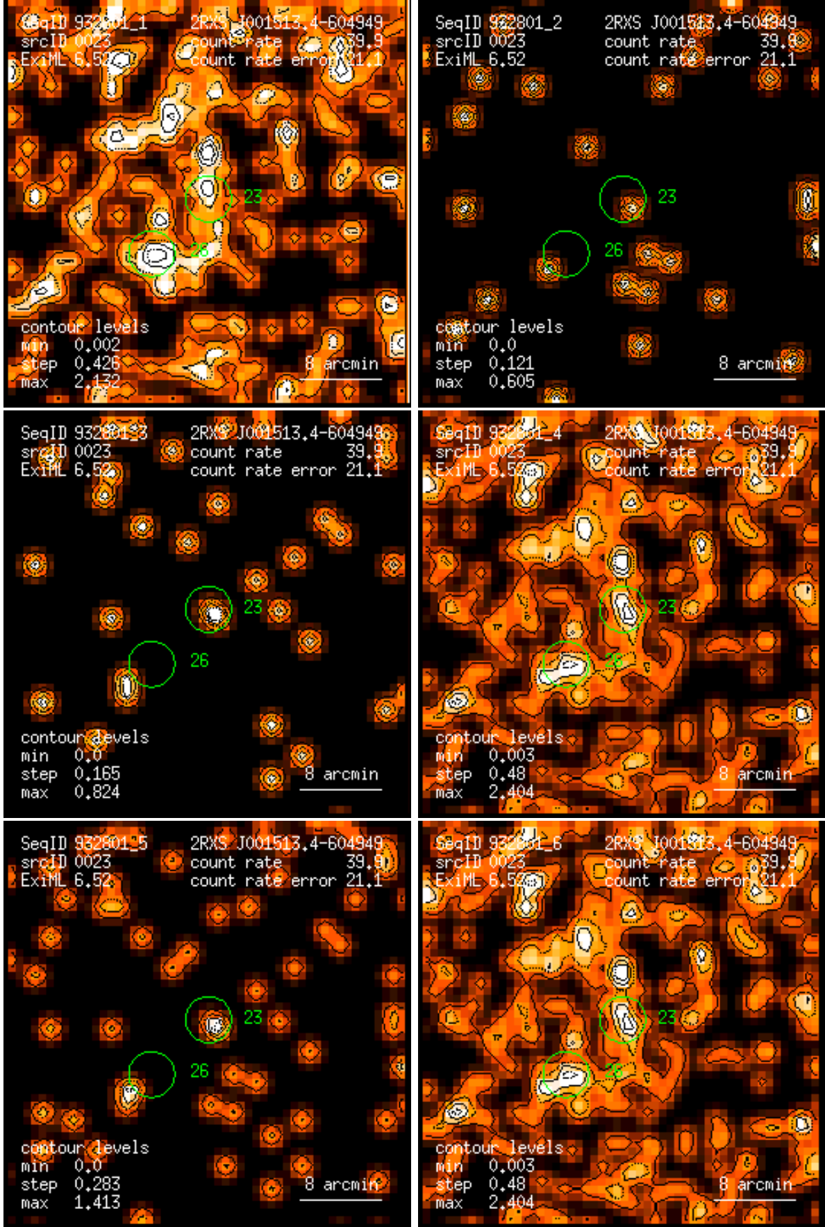
Figure 23: RASS 932801: detection 0023: band rate images, Gaussian filter: (1) PSPC channels 11 – 41, (2) 52 – 90, (3) 91 – 201, (4) 11 – 235, (5) 52 – 201, (6) 11 – 201. Broad band rates in counts/ks. Band rate contour levels in counts/ks/arcmin 2 .
