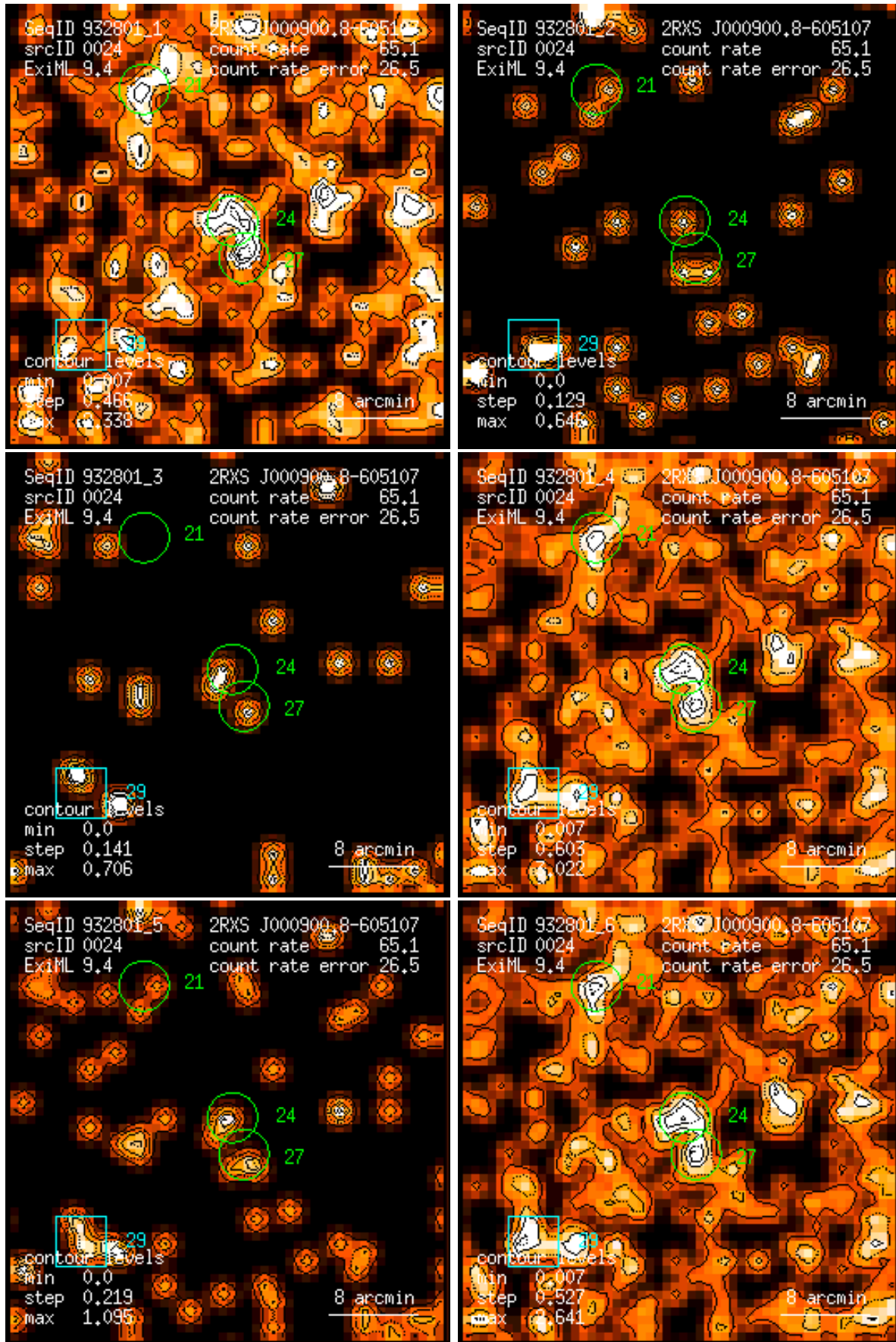
Figure 24: RASS 932801: detection 0024: band rate images, Gaussian filter: (1) PSPC channels 11 – 41, (2) 52 – 90, (3) 91 – 201, (4) 11 – 235, (5) 52 – 201, (6) 11 – 201. Broad band rates in counts/ks. Band rate contour levels in counts/ks/arcmin 2 .
