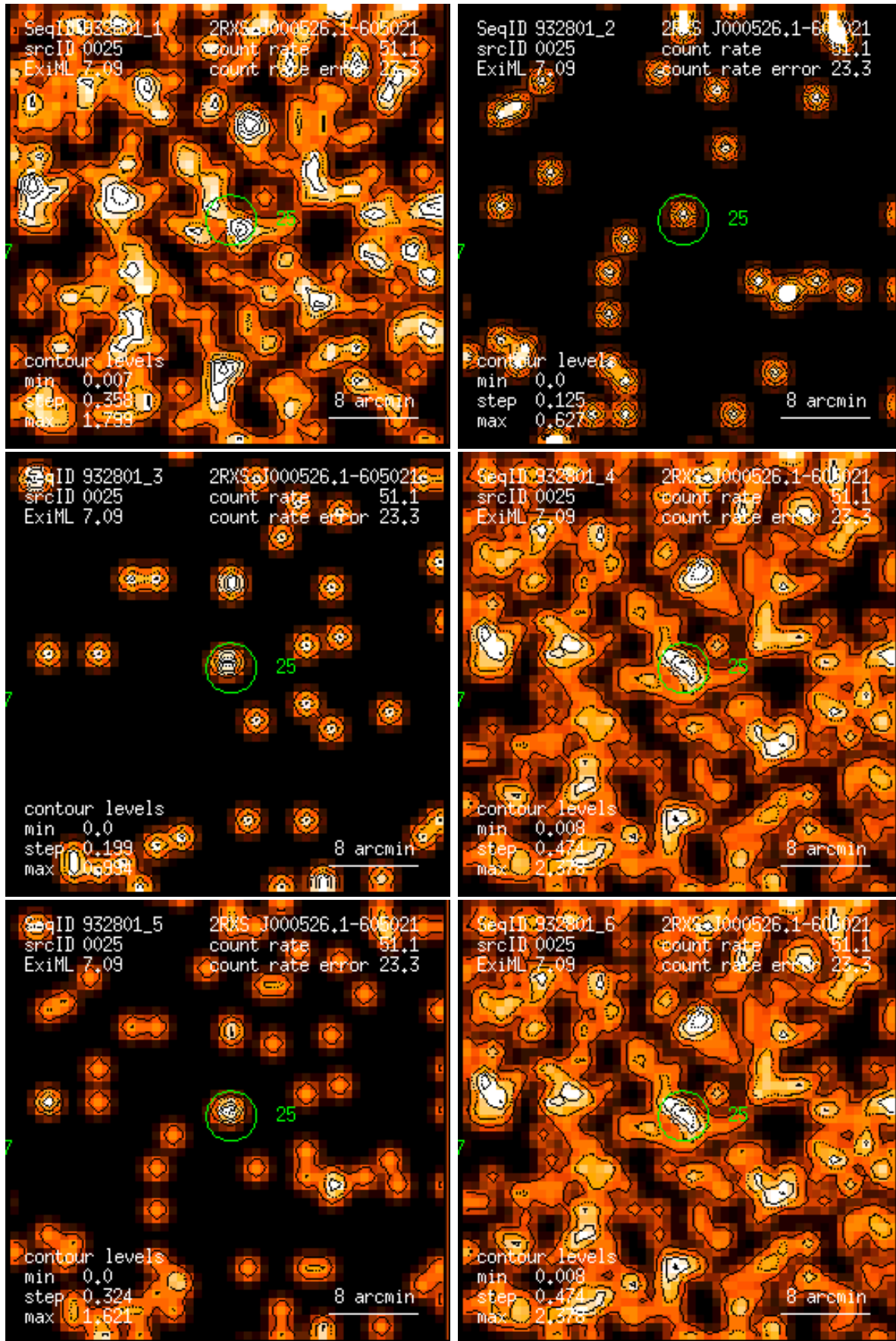
Figure 25: RASS 932801: detection 0025: band rate images, Gaussian filter: (1) PSPC channels 11 – 41, (2) 52 – 90, (3) 91 – 201, (4) 11 – 235, (5) 52 – 201, (6) 11 – 201. Broad band rates in counts/ks. Band rate contour levels in counts/ks/arcmin 2 .
