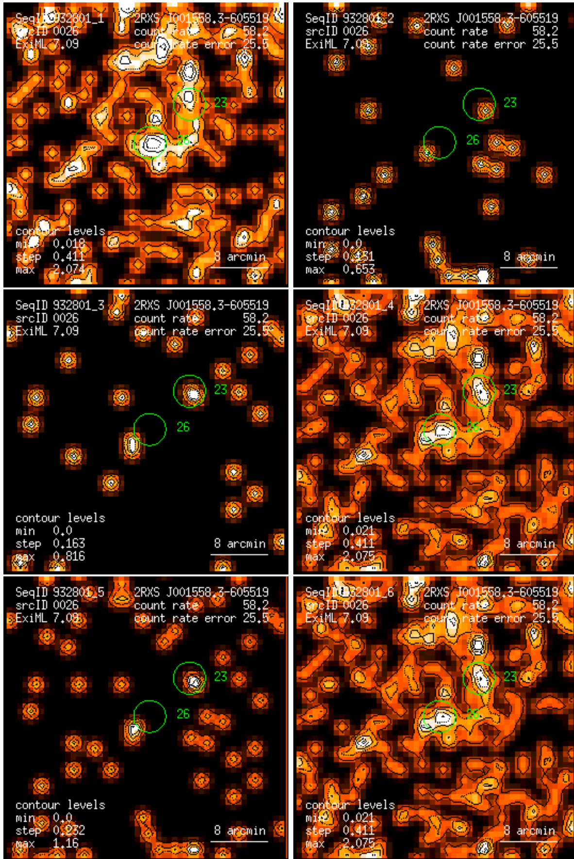
Figure 26: RASS 932801: detection 0026: band rate images, Gaussian filter: (1) PSPC channels 11 – 41, (2) 52 – 90, (3) 91 – 201, (4) 11 – 235, (5) 52 – 201, (6) 11 – 201. Broad band rates in counts/ks. Band rate contour levels in counts/ks/arcmin 2 .
