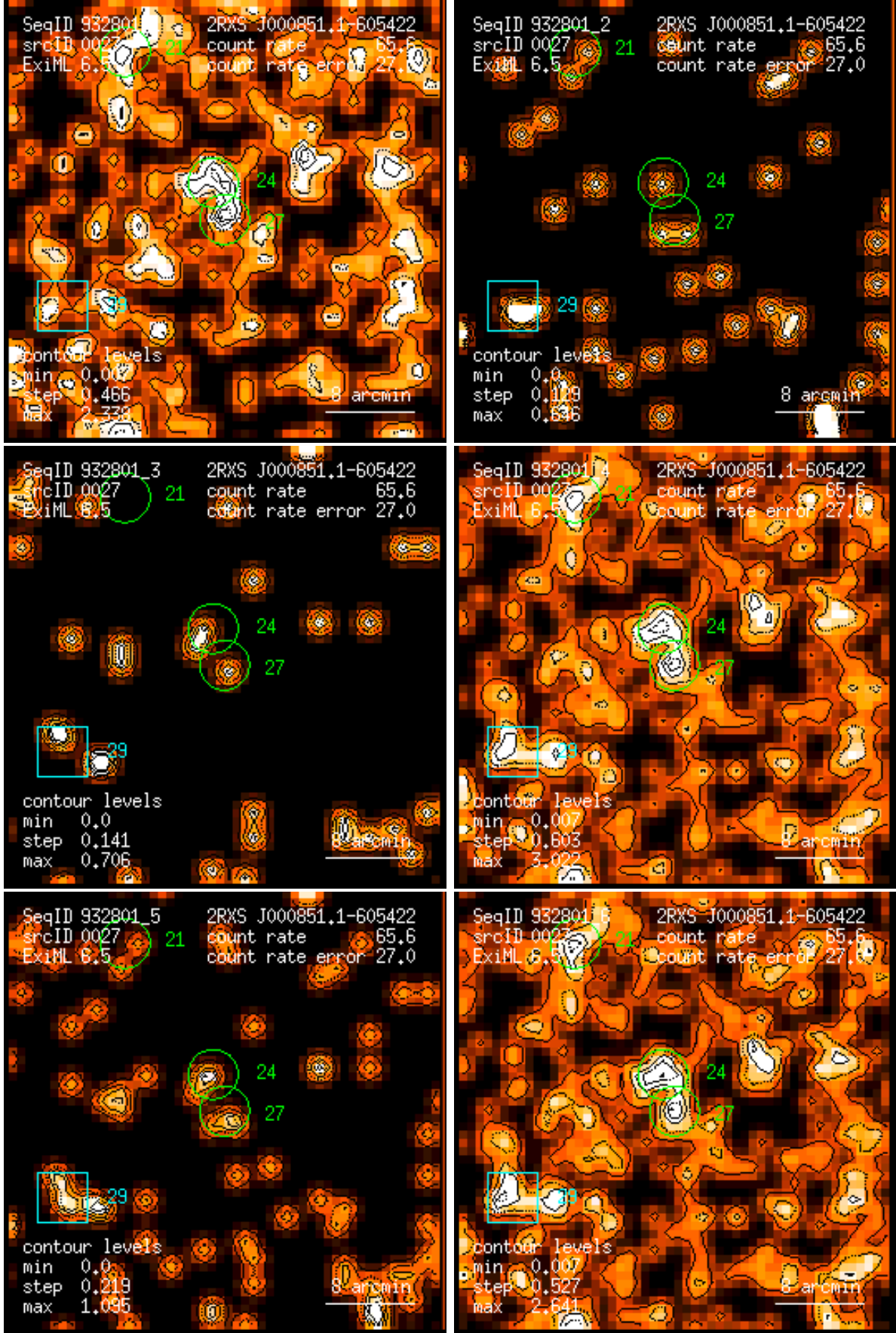
Figure 27: RASS 932801: detection 0027: band rate images, Gaussian filter: (1) PSPC channels 11 – 41, (2) 52 – 90, (3) 91 – 201, (4) 11 – 235, (5) 52 – 201, (6) 11 – 201. Broad band rates in counts/ks. Band rate contour levels in counts/ks/arcmin 2 .
