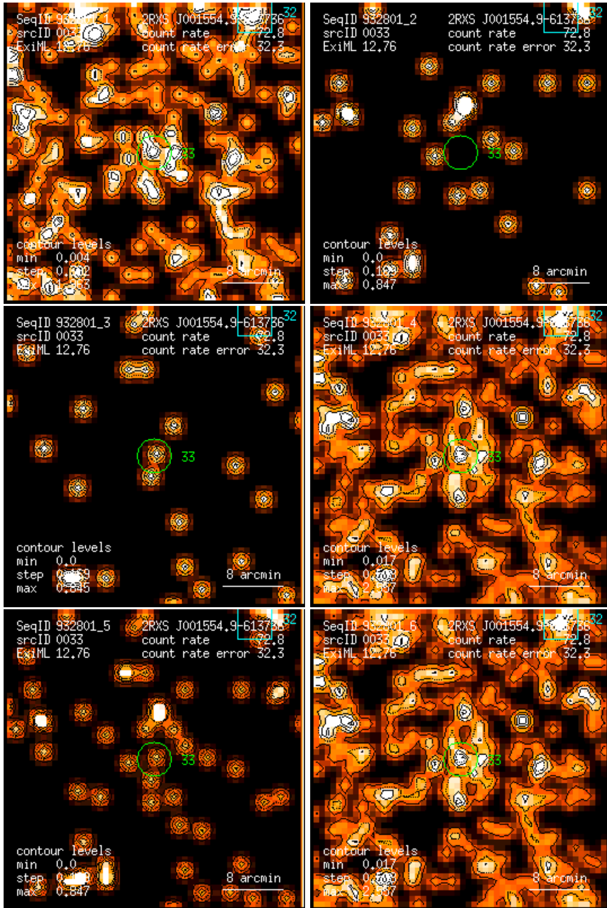
Figure 33: RASS 932801: detection 0033: band rate images, Gaussian filter: (1) PSPC channels 11 – 41, (2) 52 – 90, (3) 91 – 201, (4) 11 – 235, (5) 52 – 201, (6) 11 – 201. Broad band rates in counts/ks. Band rate contour levels in counts/ks/arcmin 2 .
