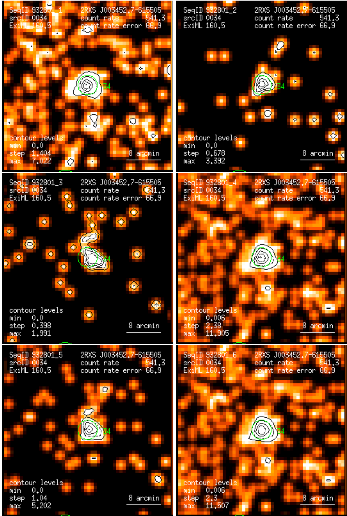
Figure 34: RASS 932801: detection 0034: band rate images, Gaussian filter: (1) PSPC channels 11 – 41, (2) 52 – 90, (3) 91 – 201, (4) 11 – 235, (5) 52 – 201, (6) 11 – 201. Broad band rates in counts/ks. Band rate contour levels in counts/ks/arcmin 2 .
