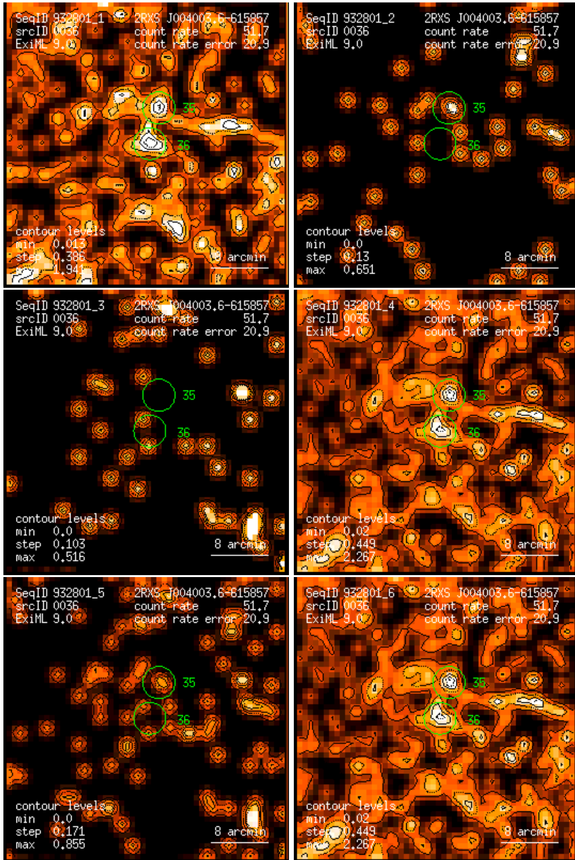
Figure 36: RASS 932801: detection 0036: band rate images, Gaussian filter: (1) PSPC channels 11 – 41, (2) 52 – 90, (3) 91 – 201, (4) 11 – 235, (5) 52 – 201, (6) 11 – 201. Broad band rates in counts/ks. Band rate contour levels in counts/ks/arcmin 2 .
