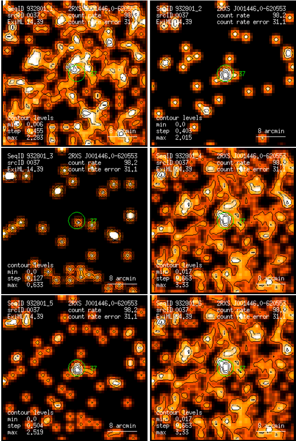
Figure 37: RASS 932801: detection 0037: band rate images, Gaussian filter: (1) PSPC channels 11 – 41, (2) 52 – 90, (3) 91 – 201, (4) 11 – 235, (5) 52 – 201, (6) 11 – 201. Broad band rates in counts/ks. Band rate contour levels in counts/ks/arcmin 2 .
