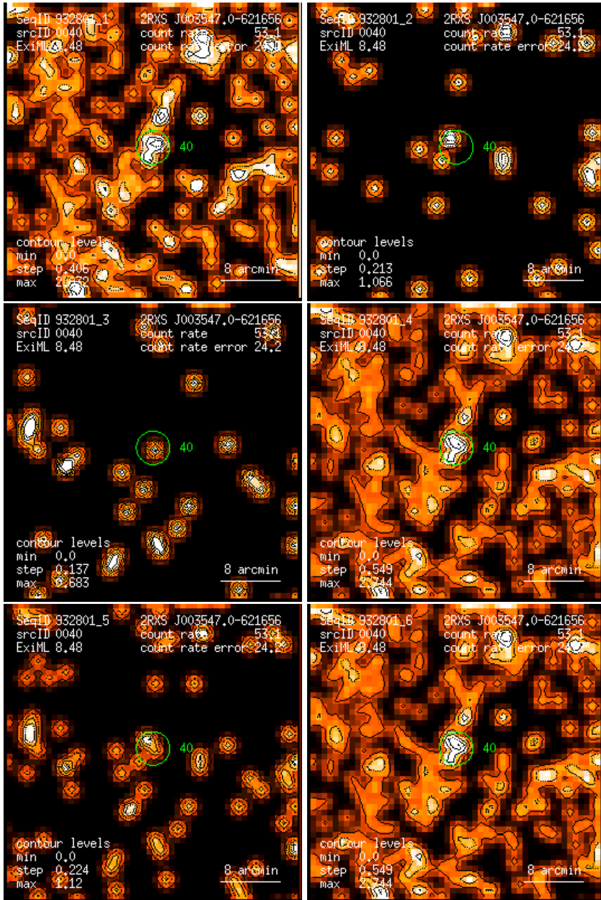
Figure 40: RASS 932801: detection 0040: band rate images, Gaussian filter: (1) PSPC channels 11 – 41, (2) 52 – 90, (3) 91 – 201, (4) 11 – 235, (5) 52 – 201, (6) 11 – 201. Broad band rates in counts/ks. Band rate contour levels in counts/ks/arcmin 2 .
