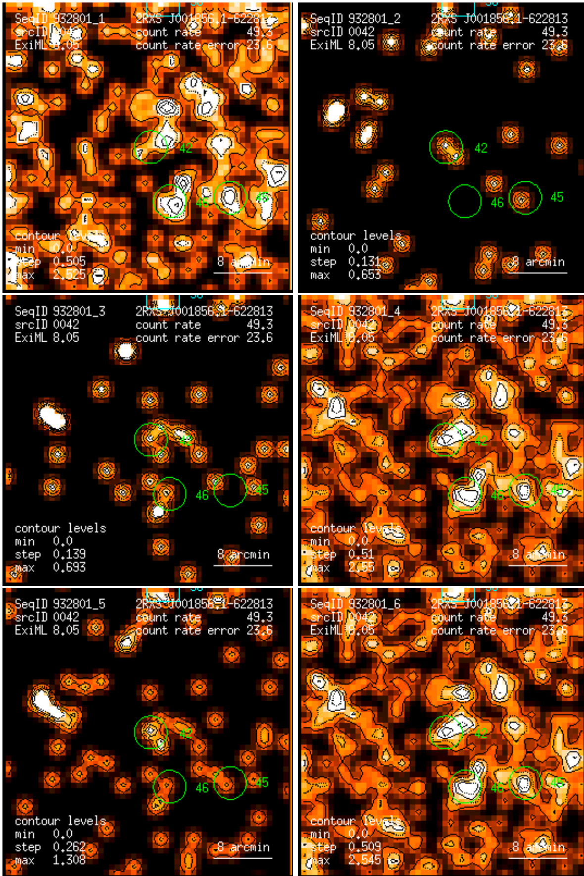
Figure 42: RASS 932801: detection 0042: band rate images, Gaussian filter: (1) PSPC channels 11 – 41, (2) 52 – 90, (3) 91 – 201, (4) 11 – 235, (5) 52 – 201, (6) 11 – 201. Broad band rates in counts/ks. Band rate contour levels in counts/ks/arcmin 2 .
