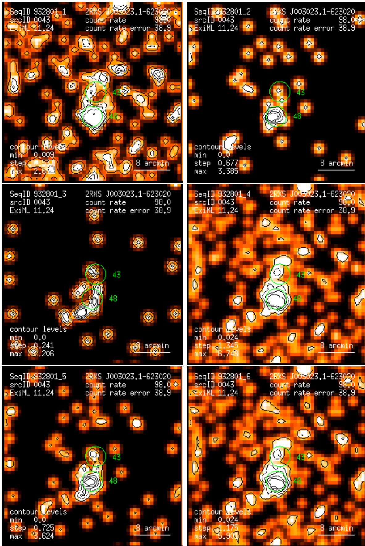
Figure 43: RASS 932801: detection 0043: band rate images, Gaussian filter: (1) PSPC channels 11 – 41, (2) 52 – 90, (3) 91 – 201, (4) 11 – 235, (5) 52 – 201, (6) 11 – 201. Broad band rates in counts/ks. Band rate contour levels in counts/ks/arcmin 2 .
