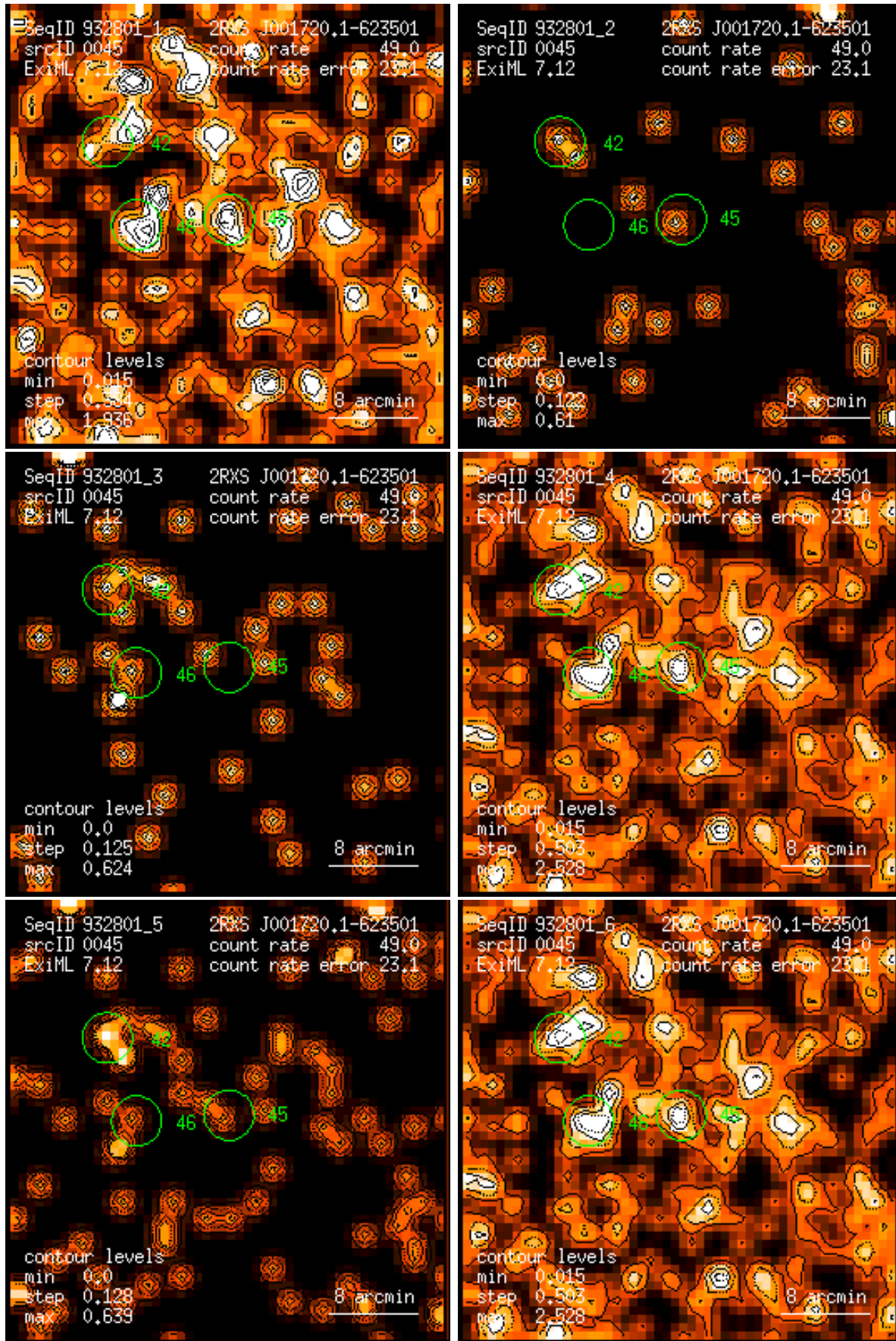
Figure 45: RASS 932801: detection 0045: band rate images, Gaussian filter: (1) PSPC channels 11 – 41, (2) 52 – 90, (3) 91 – 201, (4) 11 – 235, (5) 52 – 201, (6) 11 – 201. Broad band rates in counts/ks. Band rate contour levels in counts/ks/arcmin 2 .
