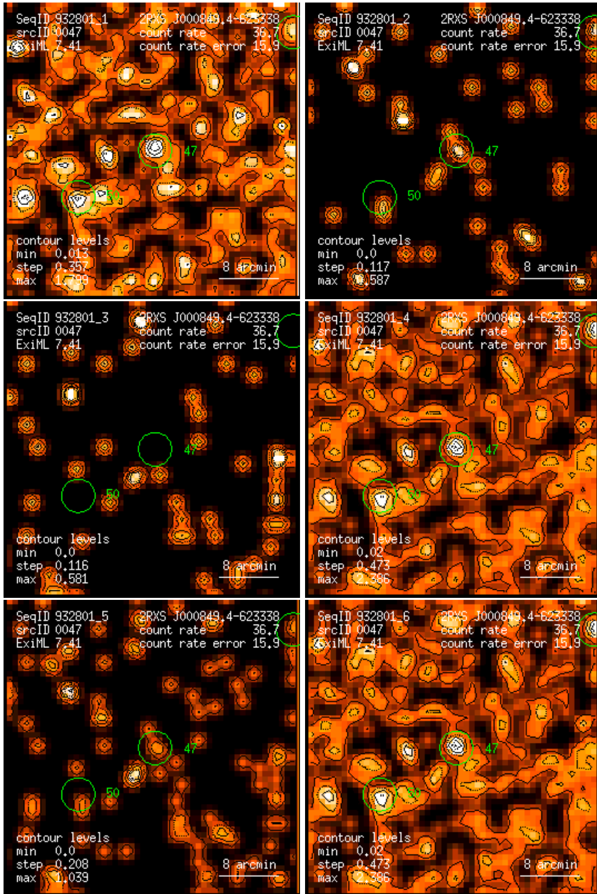
Figure 47: RASS 932801: detection 0047: band rate images, Gaussian filter: (1) PSPC channels 11 – 41, (2) 52 – 90, (3) 91 – 201, (4) 11 – 235, (5) 52 – 201, (6) 11 – 201. Broad band rates in counts/ks. Band rate contour levels in counts/ks/arcmin 2 .
