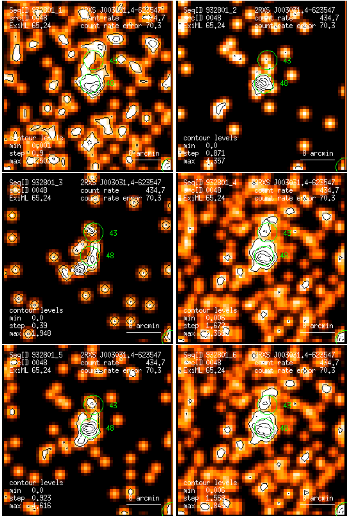
Figure 48: RASS 932801: detection 0048: band rate images, Gaussian filter: (1) PSPC channels 11 – 41, (2) 52 – 90, (3) 91 – 201, (4) 11 – 235, (5) 52 – 201, (6) 11 – 201. Broad band rates in counts/ks. Band rate contour levels in counts/ks/arcmin 2 .
