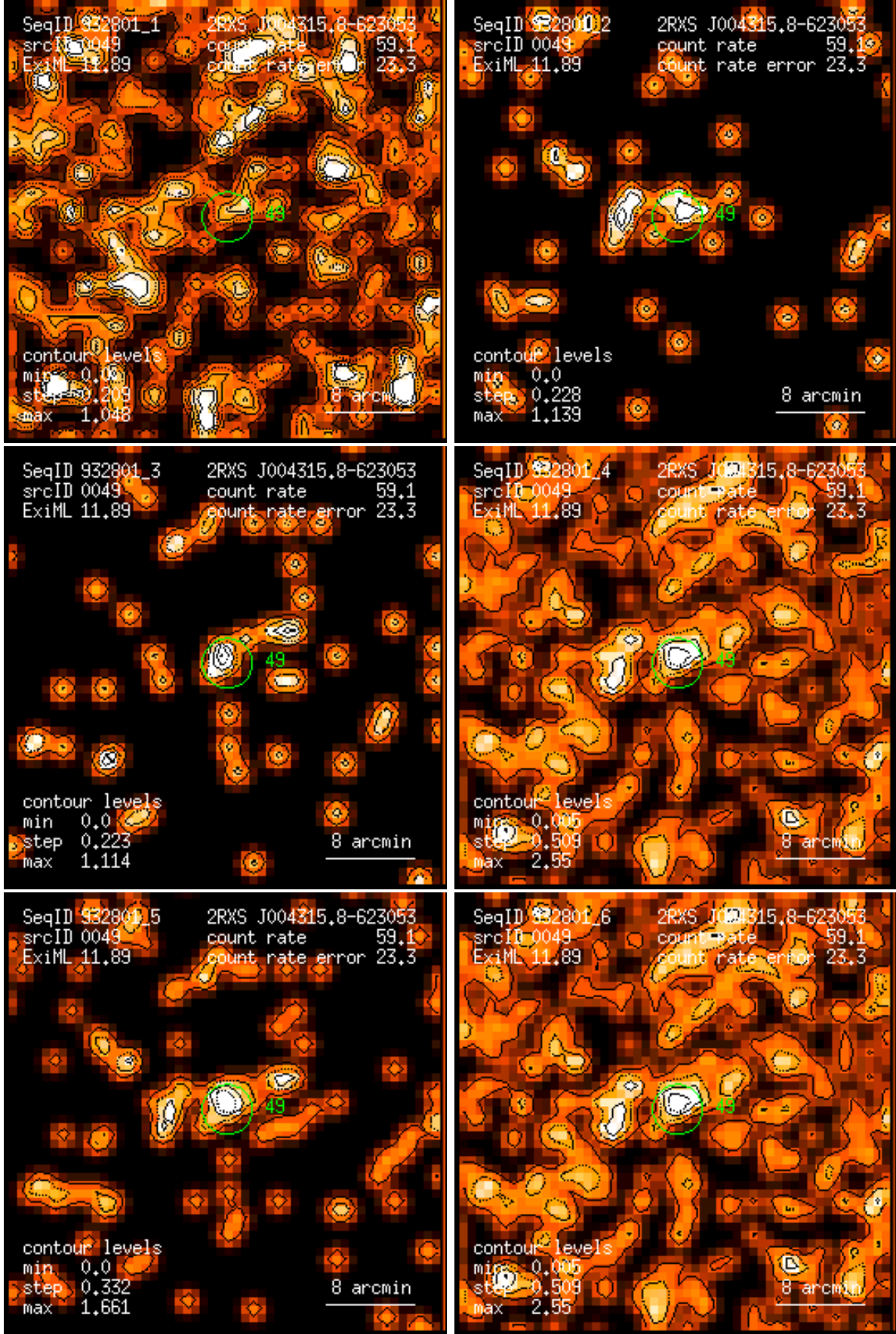
Figure 49: RASS 932801: detection 0049: band rate images, Gaussian filter: (1) PSPC channels 11 – 41, (2) 52 – 90, (3) 91 – 201, (4) 11 – 235, (5) 52 – 201, (6) 11 – 201. Broad band rates in counts/ks. Band rate contour levels in counts/ks/arcmin 2 .
