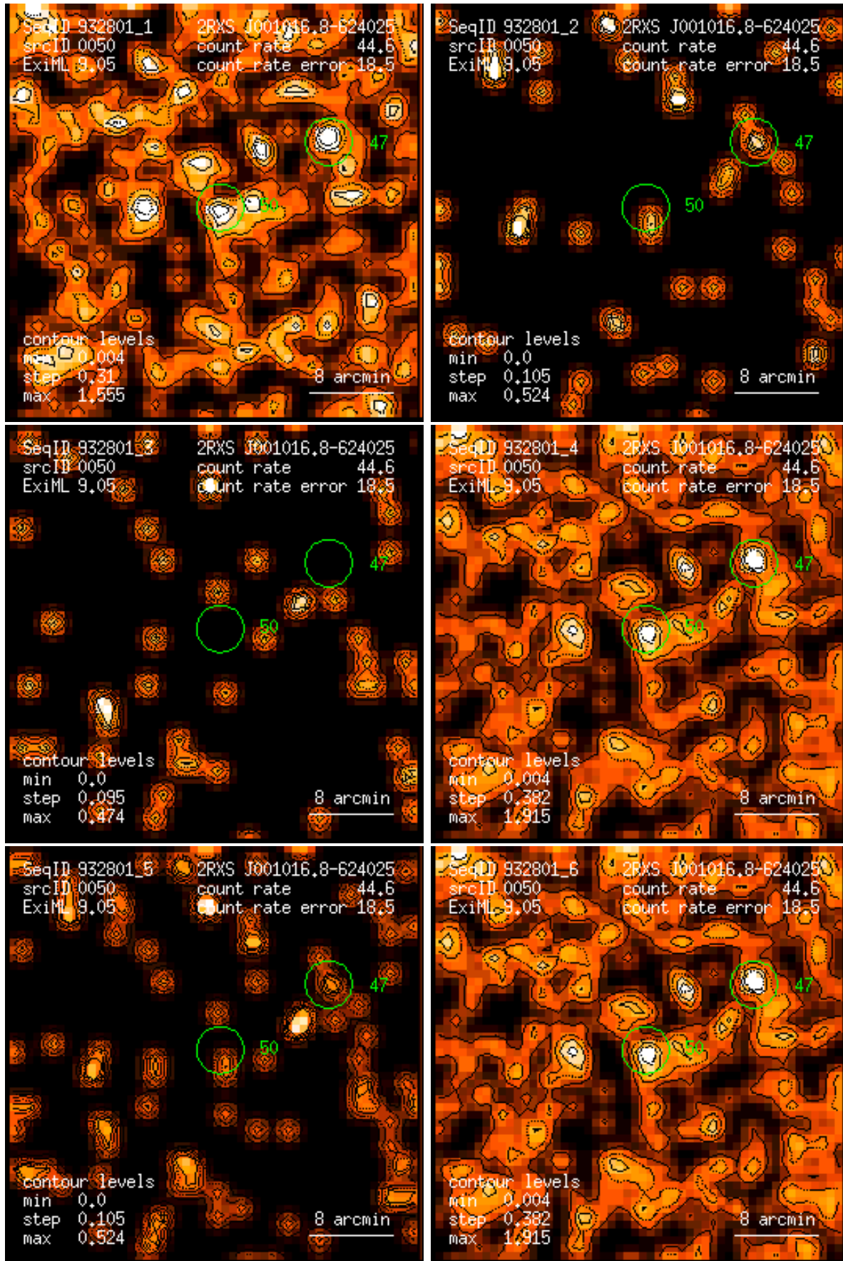
Figure 50: RASS 932801: detection 0050: band rate images, Gaussian filter: (1) PSPC channels 11 – 41, (2) 52 – 90, (3) 91 – 201, (4) 11 – 235, (5) 52 – 201, (6) 11 – 201. Broad band rates in counts/ks. Band rate contour levels in counts/ks/arcmin 2 .
