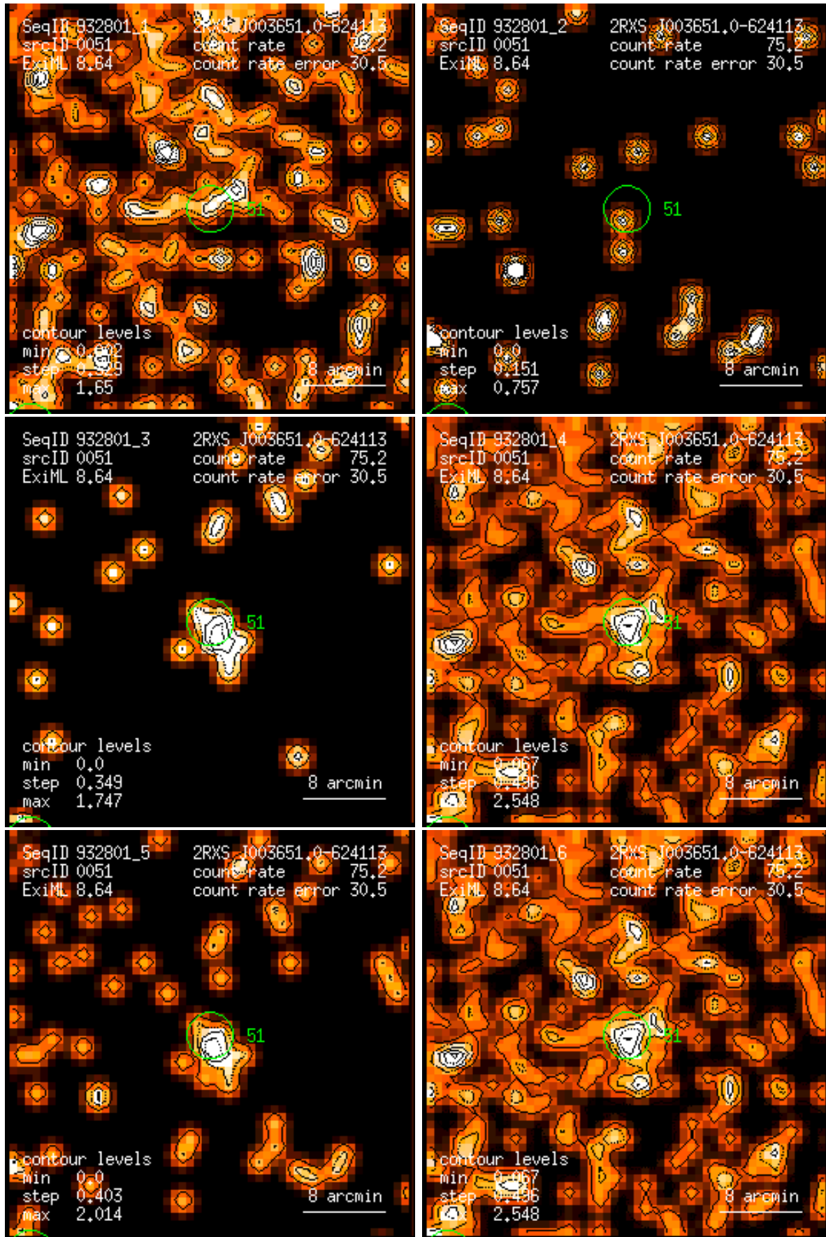
Figure 51: RASS 932801: detection 0051: band rate images, Gaussian filter: (1) PSPC channels 11 – 41, (2) 52 – 90, (3) 91 – 201, (4) 11 – 235, (5) 52 – 201, (6) 11 – 201. Broad band rates in counts/ks. Band rate contour levels in counts/ks/arcmin 2 .
