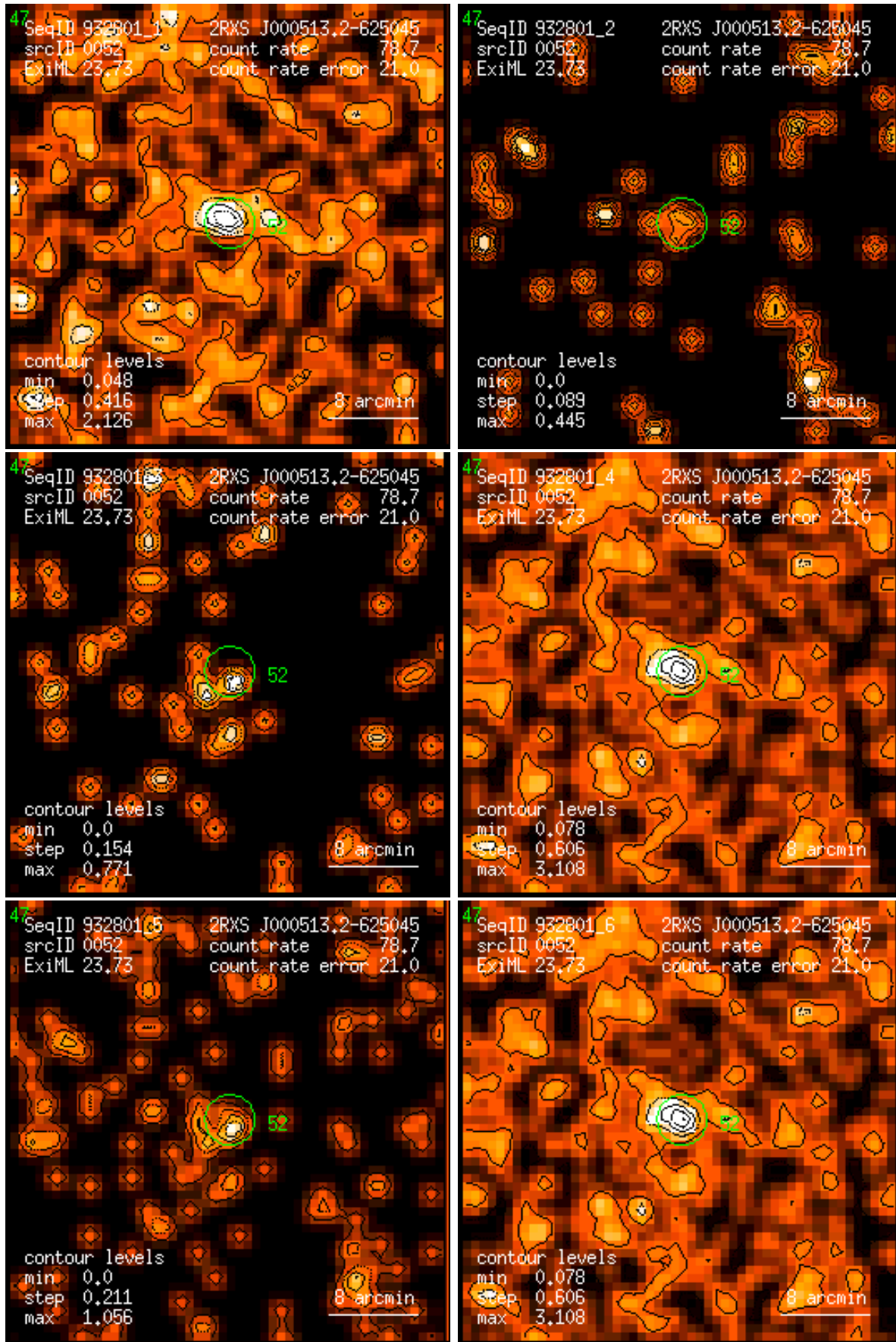
Figure 52: RASS 932801: detection 0052: band rate images, Gaussian filter: (1) PSPC channels 11 – 41, (2) 52 – 90, (3) 91 – 201, (4) 11 – 235, (5) 52 – 201, (6) 11 – 201. Broad band rates in counts/ks. Band rate contour levels in counts/ks/arcmin 2 .
