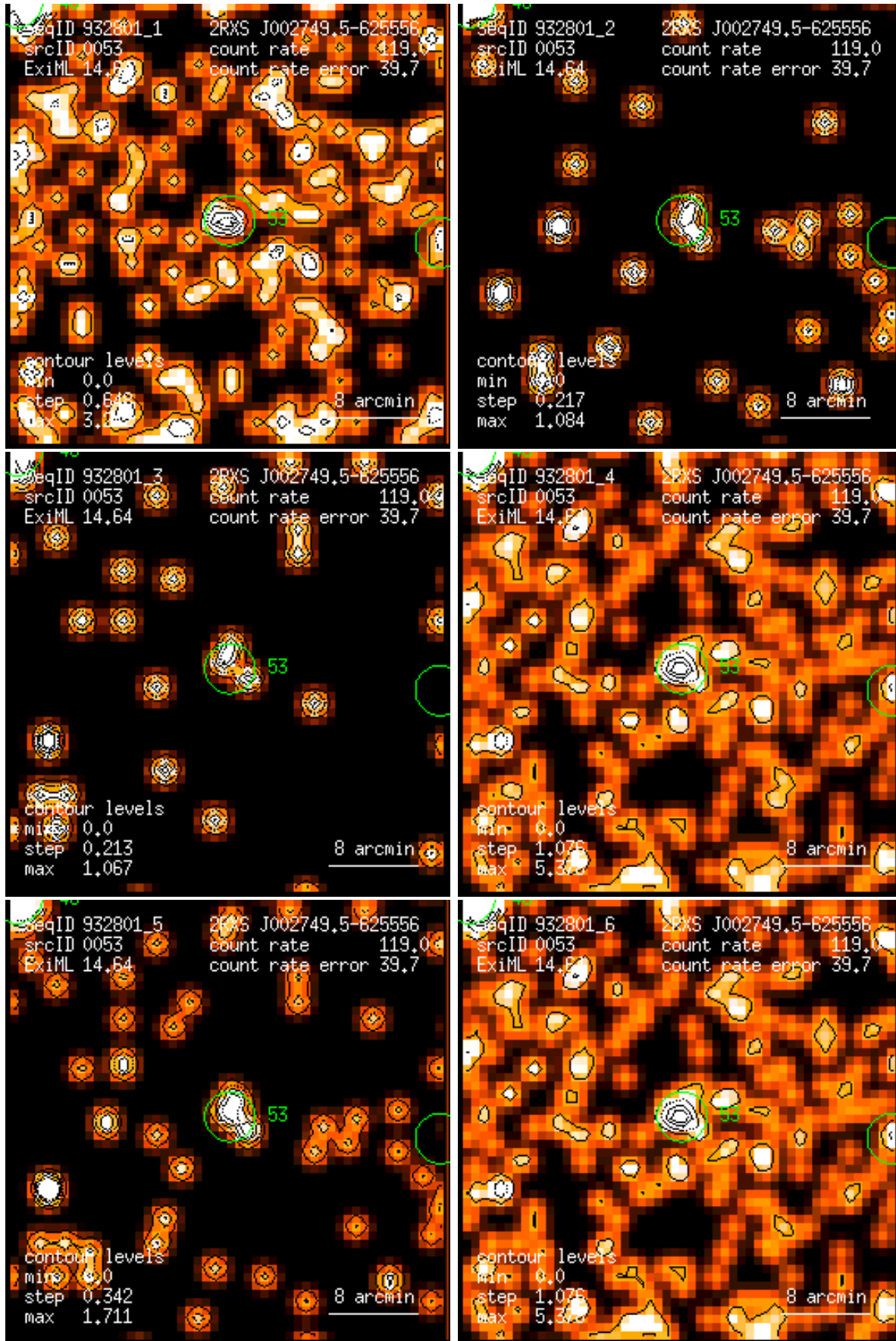
Figure 53: RASS 932801: detection 0053: band rate images, Gaussian filter: (1) PSPC channels 11 – 41, (2) 52 – 90, (3) 91 – 201, (4) 11 – 235, (5) 52 – 201, (6) 11 – 201. Broad band rates in counts/ks. Band rate contour levels in counts/ks/arcmin 2 .
