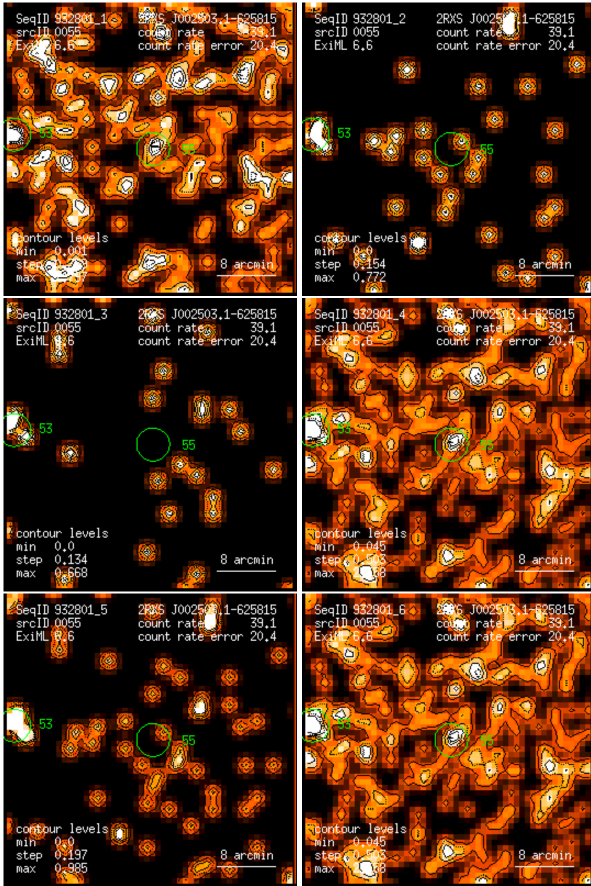
Figure 55: RASS 932801: detection 0055: band rate images, Gaussian filter: (1) PSPC channels 11 – 41, (2) 52 – 90, (3) 91 – 201, (4) 11 – 235, (5) 52 – 201, (6) 11 – 201. Broad band rates in counts/ks. Band rate contour levels in counts/ks/arcmin 2 .
