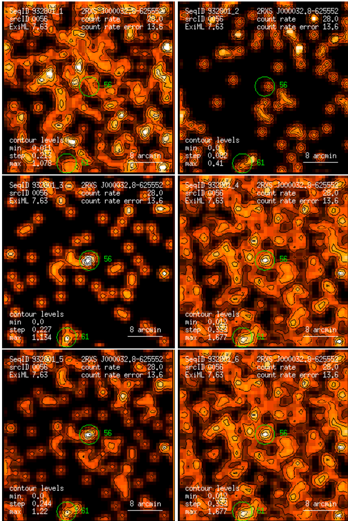
Figure 56: RASS 932801: detection 0056: band rate images, Gaussian filter: (1) PSPC channels 11 – 41, (2) 52 – 90, (3) 91 – 201, (4) 11 – 235, (5) 52 – 201, (6) 11 – 201. Broad band rates in counts/ks. Band rate contour levels in counts/ks/arcmin 2 .
