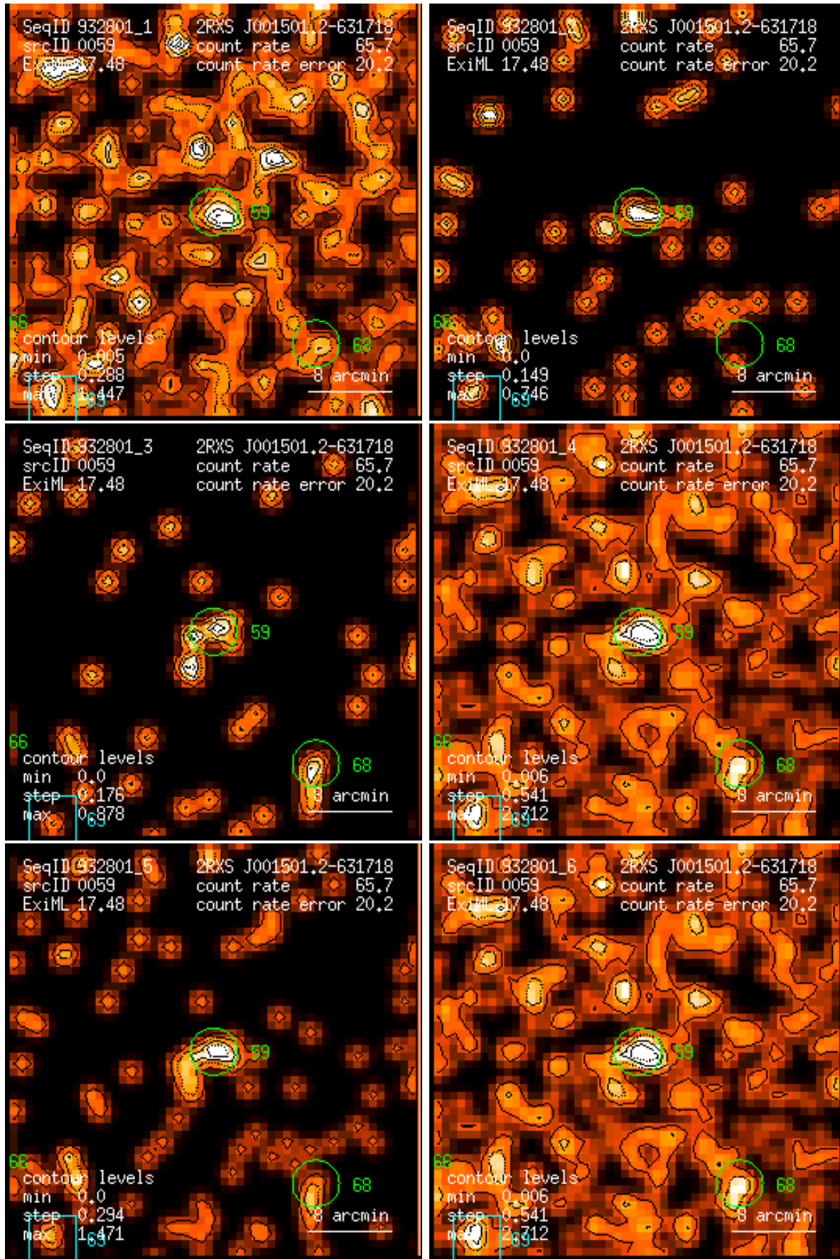
Figure 59: RASS 932801: detection 0059: band rate images, Gaussian filter: (1) PSPC channels 11 – 41, (2) 52 – 90, (3) 91 – 201, (4) 11 – 235, (5) 52 – 201, (6) 11 – 201. Broad band rates in counts/ks. Band rate contour levels in counts/ks/arcmin 2 .
