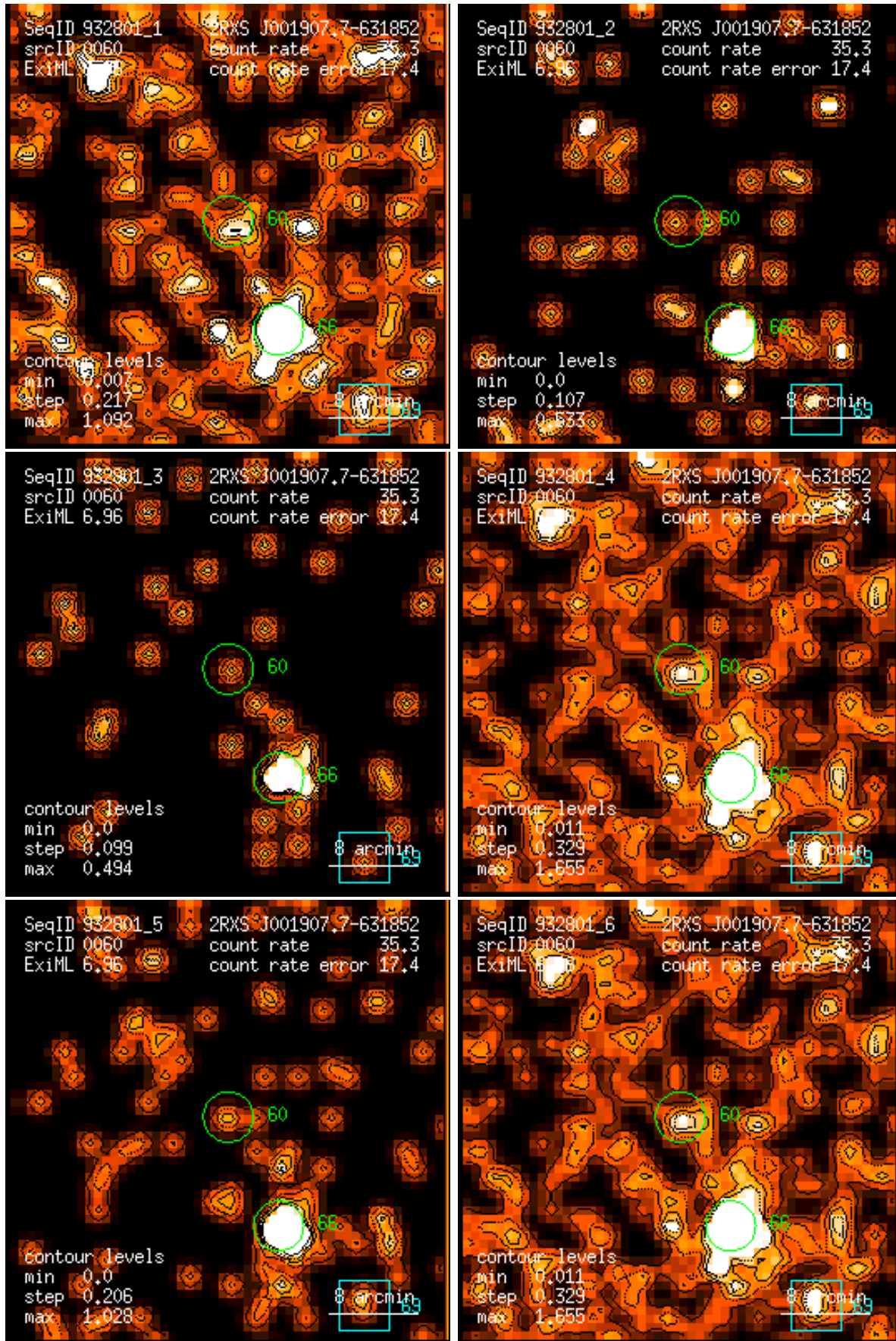
Figure 60: RASS 932801: detection 0060: band rate images, Gaussian filter: (1) PSPC channels 11 – 41, (2) 52 – 90, (3) 91 – 201, (4) 11 – 235, (5) 52 – 201, (6) 11 – 201. Broad band rates in counts/ks. Band rate contour levels in counts/ks/arcmin 2 .
