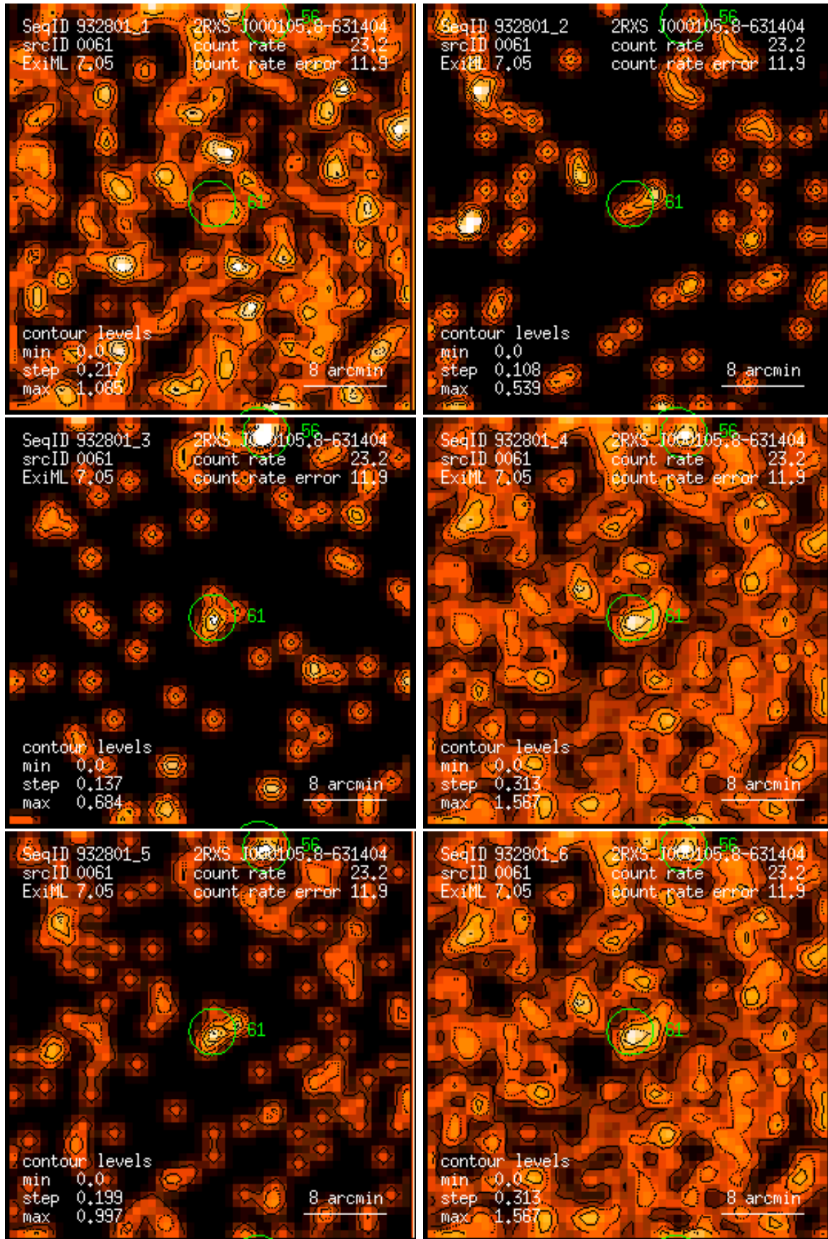
Figure 61: RASS 932801: detection 0061: band rate images, Gaussian filter: (1) PSPC channels 11 – 41, (2) 52 – 90, (3) 91 – 201, (4) 11 – 235, (5) 52 – 201, (6) 11 – 201. Broad band rates in counts/ks. Band rate contour levels in counts/ks/arcmin 2 .
